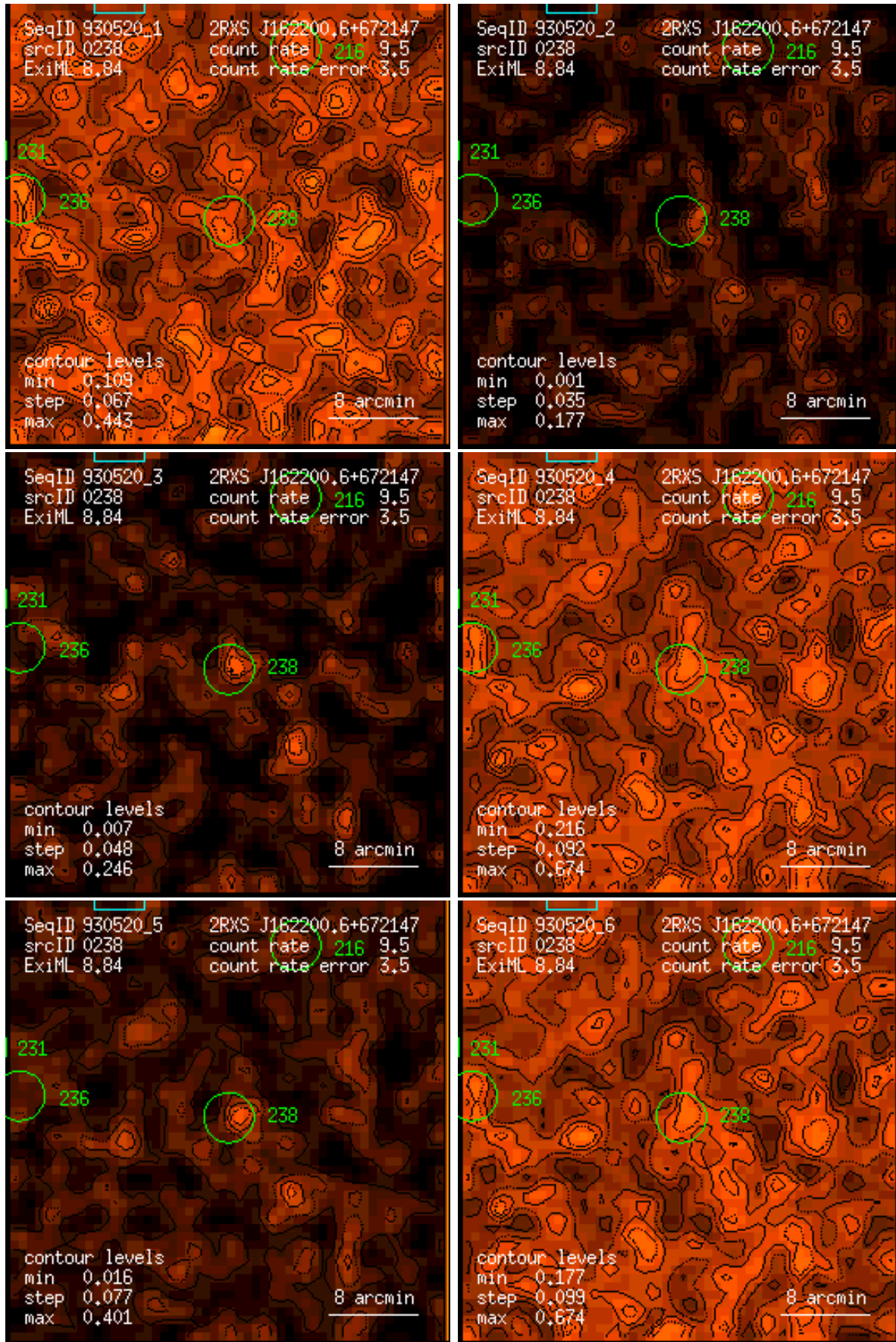
Figure 238: RASS 930520: detection 0238: band rate images, Gaussian filter: (1) PSPC channels 11 – 41, (2) 52 – 90, (3) 91 – 201, (4) 11 – 235, (5) 52 – 201, (6) 11 – 201. Broad band rates in counts/ks. Band rate contour levels in counts/ks/arcmin 2 .
