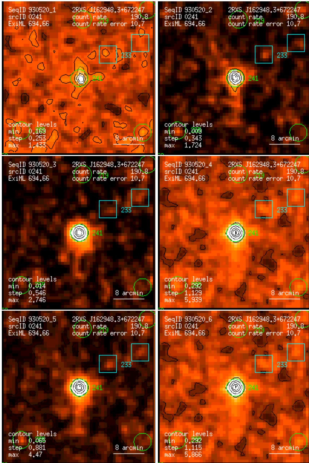
Figure 241: RASS 930520: detection 0241: band rate images, Gaussian filter: (1) PSPC channels 11 – 41, (2) 52 – 90, (3) 91 – 201, (4) 11 – 235, (5) 52 – 201, (6) 11 – 201. Broad band rates in counts/ks. Band rate contour levels in counts/ks/arcmin 2 .
