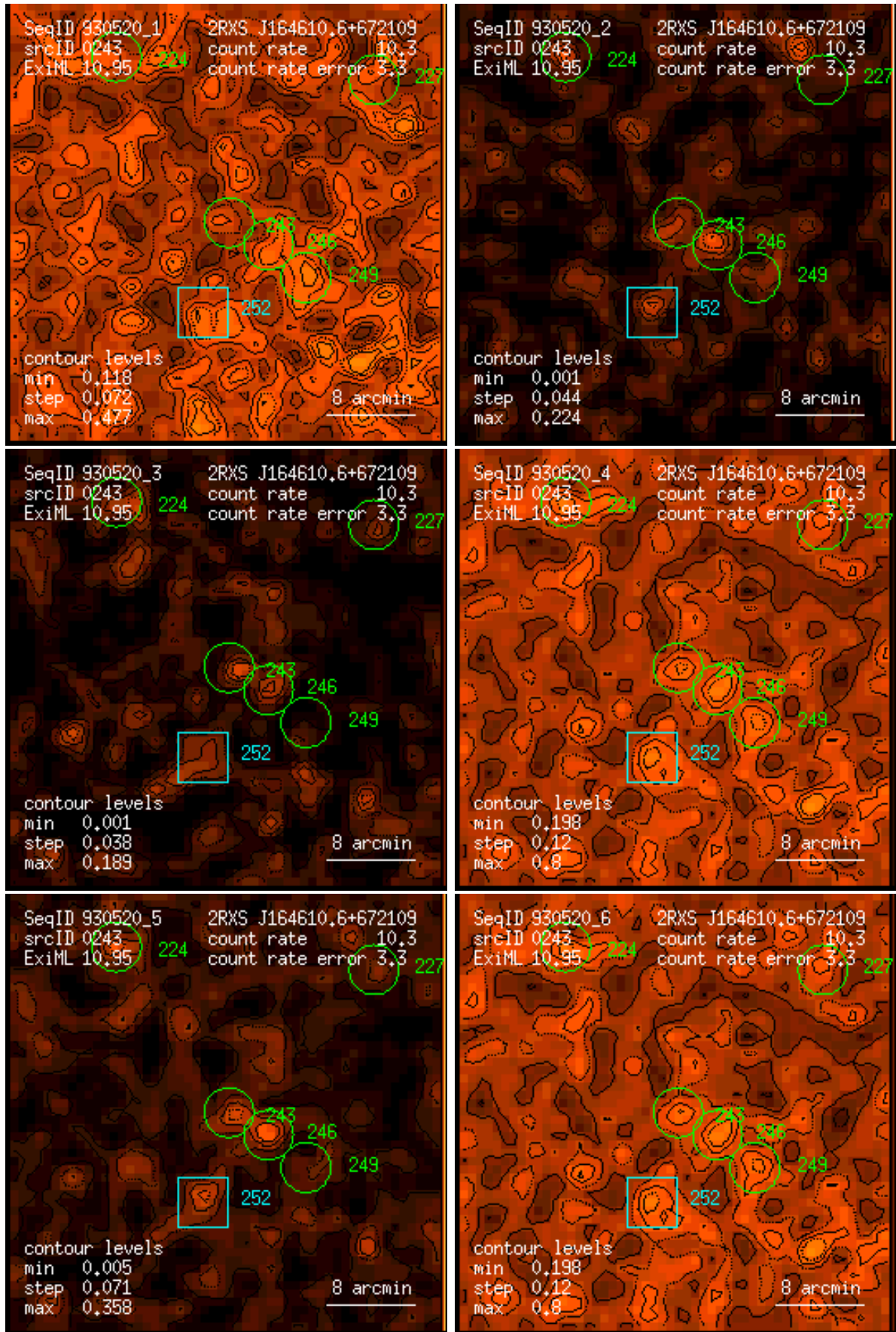
Figure 243: RASS 930520: detection 0243: band rate images, Gaussian filter: (1) PSPC channels 11 – 41, (2) 52 – 90, (3) 91 – 201, (4) 11 – 235, (5) 52 – 201, (6) 11 – 201. Broad band rates in counts/ks. Band rate contour levels in counts/ks/arcmin 2 .
