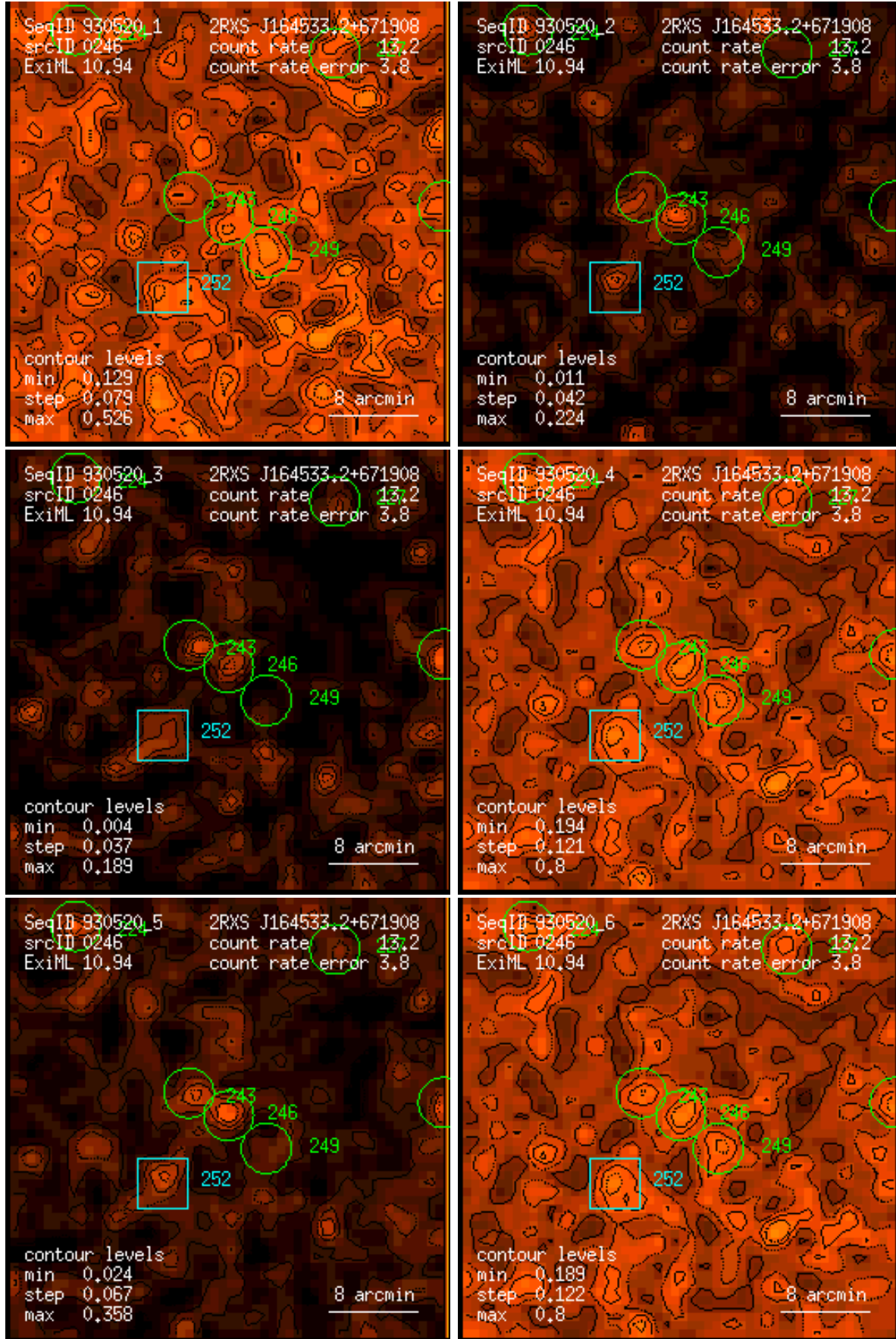
Figure 246: RASS 930520: detection 0246: band rate images, Gaussian filter: (1) PSPC channels 11 – 41, (2) 52 – 90, (3) 91 – 201, (4) 11 – 235, (5) 52 – 201, (6) 11 – 201. Broad band rates in counts/ks. Band rate contour levels in counts/ks/arcmin 2 .
