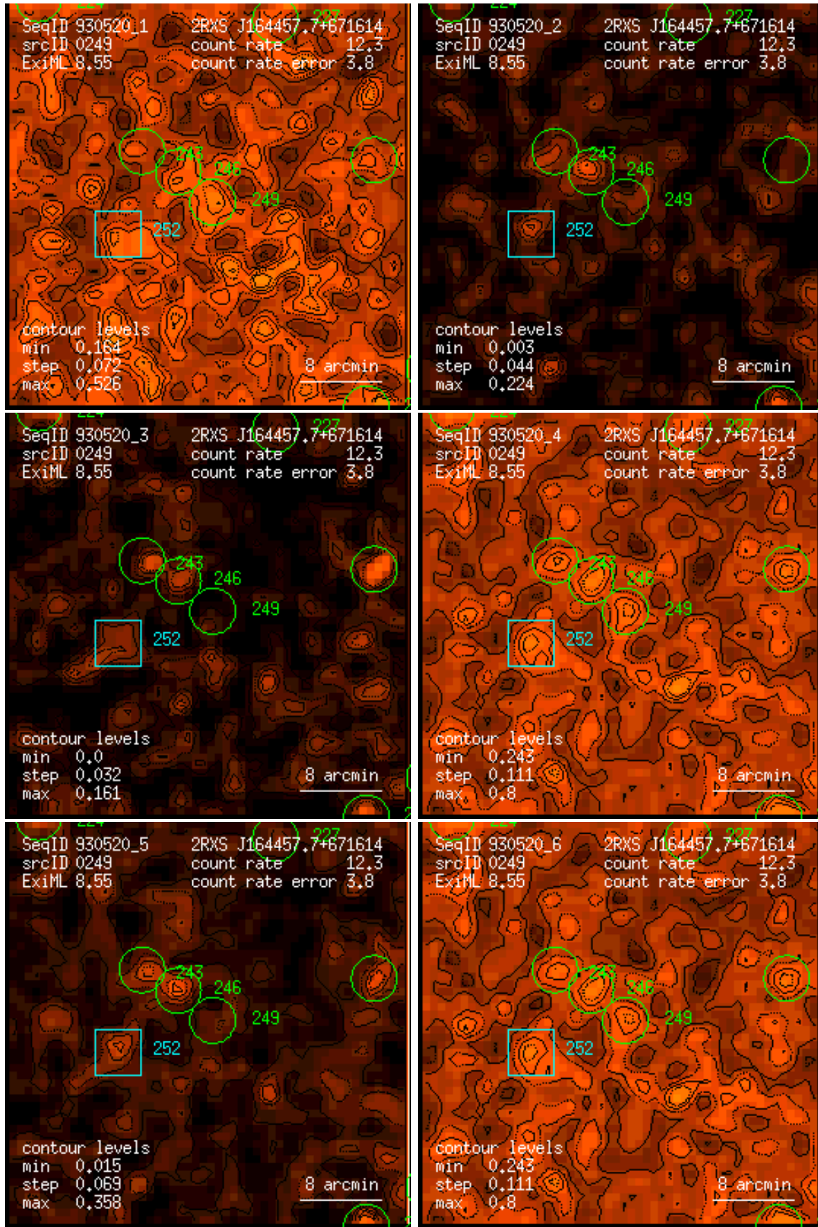
Figure 249: RASS 930520: detection 0249: band rate images, Gaussian filter: (1) PSPC channels 11 – 41, (2) 52 – 90, (3) 91 – 201, (4) 11 – 235, (5) 52 – 201, (6) 11 – 201. Broad band rates in counts/ks. Band rate contour levels in counts/ks/arcmin 2 .
