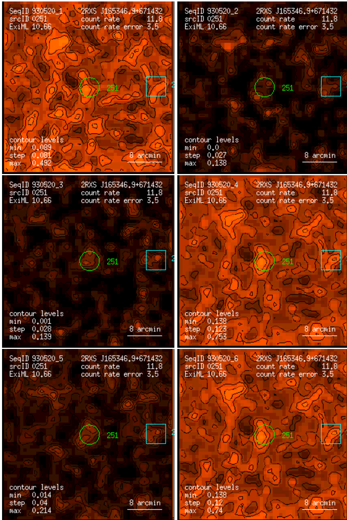
Figure 251: RASS 930520: detection 0251: band rate images, Gaussian filter: (1) PSPC channels 11 – 41, (2) 52 – 90, (3) 91 – 201, (4) 11 – 235, (5) 52 – 201, (6) 11 – 201. Broad band rates in counts/ks. Band rate contour levels in counts/ks/arcmin 2 .
