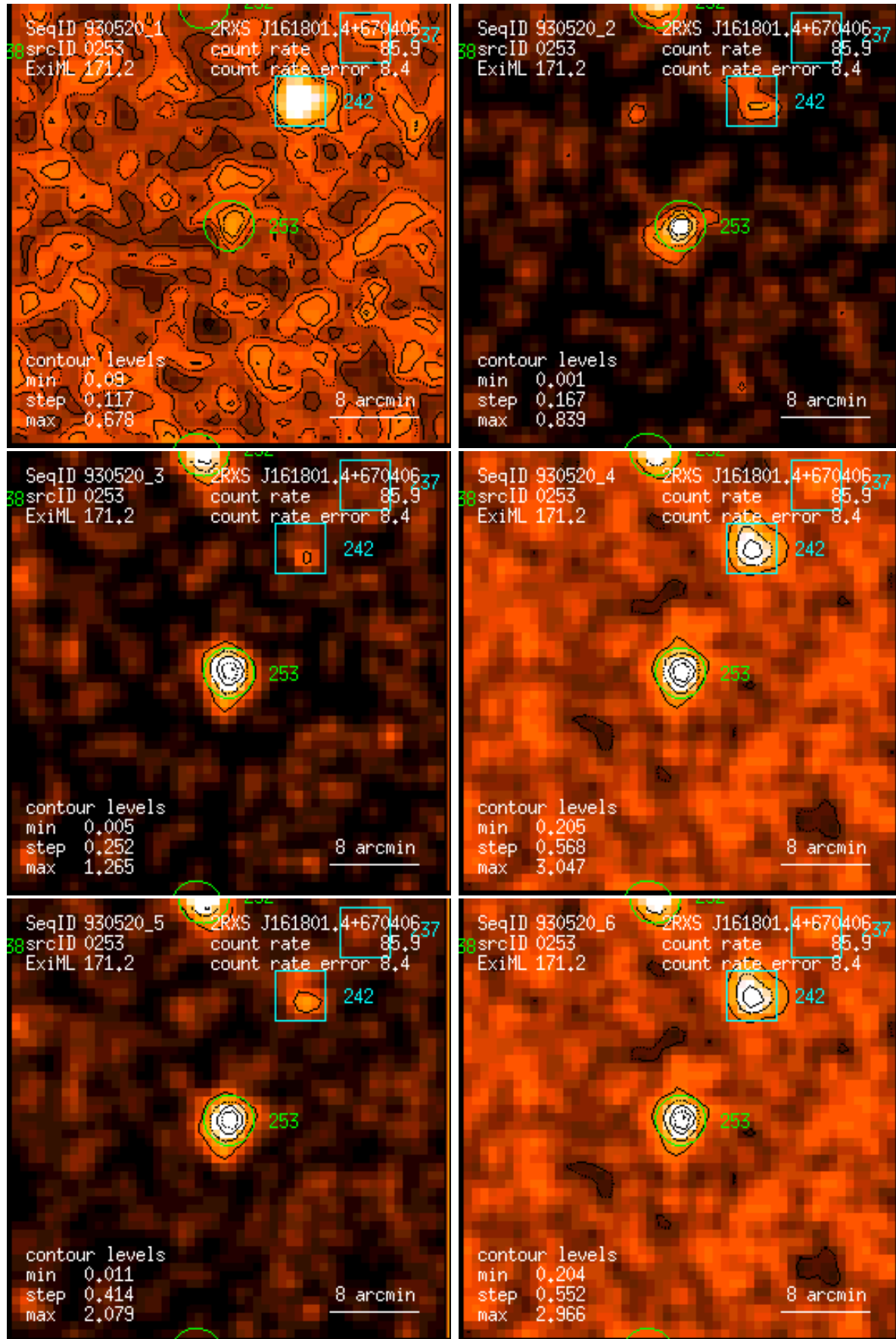
Figure 253: RASS 930520: detection 0253: band rate images, Gaussian filter: (1) PSPC channels 11 – 41, (2) 52 – 90, (3) 91 – 201, (4) 11 – 235, (5) 52 – 201, (6) 11 – 201. Broad band rates in counts/ks. Band rate contour levels in counts/ks/arcmin 2 .
