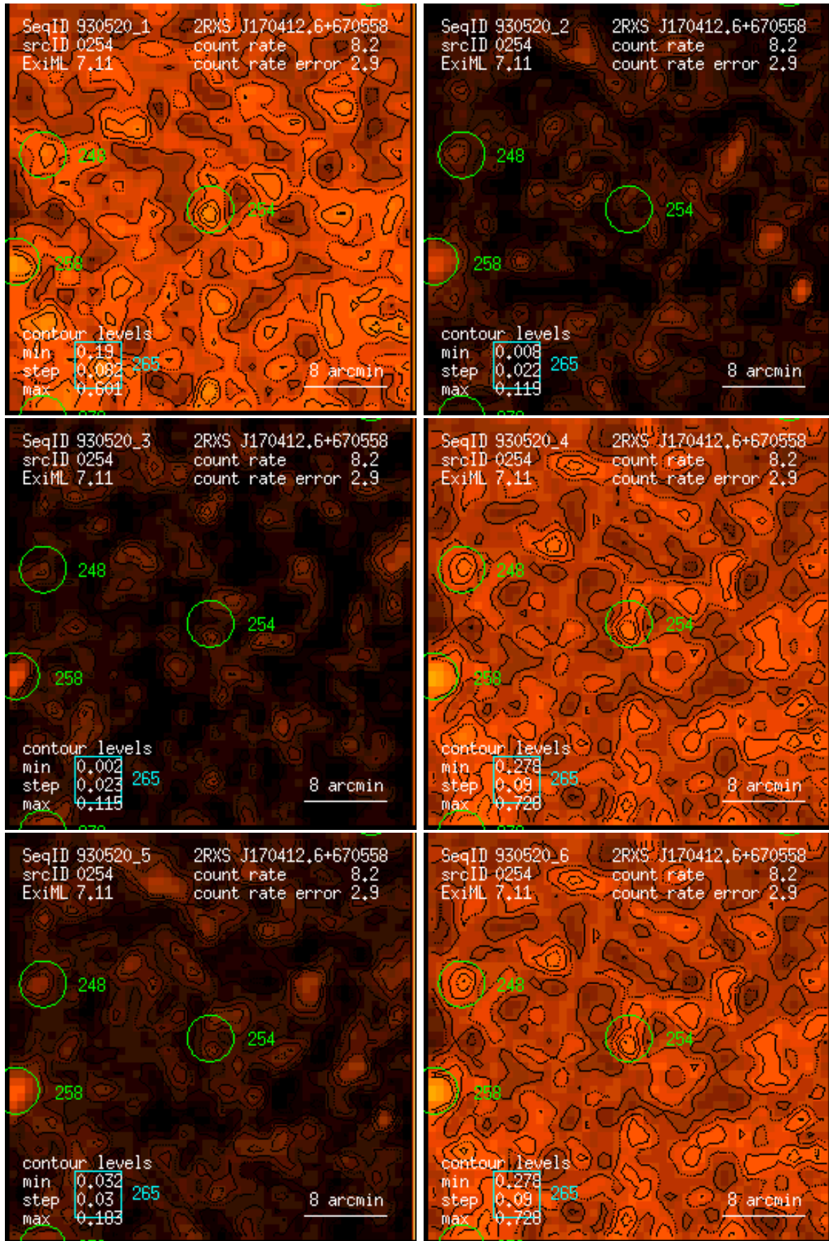
Figure 254: RASS 930520: detection 0254: band rate images, Gaussian filter: (1) PSPC channels 11 – 41, (2) 52 – 90, (3) 91 – 201, (4) 11 – 235, (5) 52 – 201, (6) 11 – 201. Broad band rates in counts/ks. Band rate contour levels in counts/ks/arcmin 2 .
