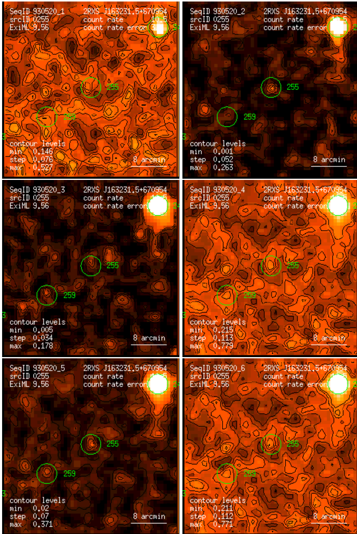
Figure 255: RASS 930520: detection 0255: band rate images, Gaussian filter: (1) PSPC channels 11 – 41, (2) 52 – 90, (3) 91 – 201, (4) 11 – 235, (5) 52 – 201, (6) 11 – 201. Broad band rates in counts/ks. Band rate contour levels in counts/ks/arcmin 2 .
