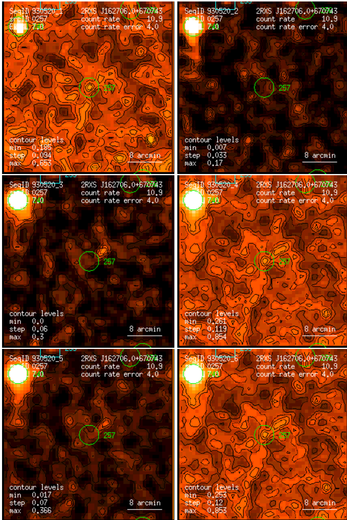
Figure 257: RASS 930520: detection 0257: band rate images, Gaussian filter: (1) PSPC channels 11 – 41, (2) 52 – 90, (3) 91 – 201, (4) 11 – 235, (5) 52 – 201, (6) 11 – 201. Broad band rates in counts/ks. Band rate contour levels in counts/ks/arcmin 2 .
