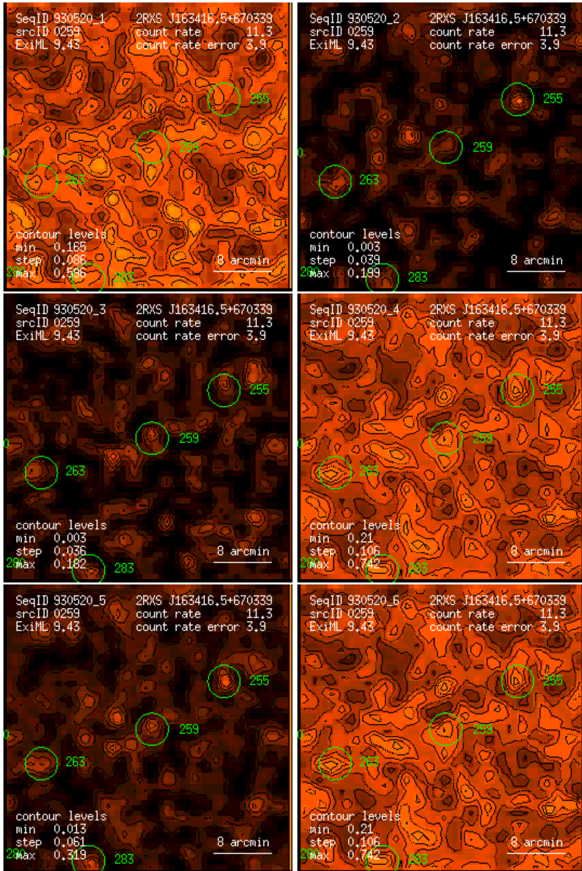
Figure 259: RASS 930520: detection 0259: band rate images, Gaussian filter: (1) PSPC channels 11 – 41, (2) 52 – 90, (3) 91 – 201, (4) 11 – 235, (5) 52 – 201, (6) 11 – 201. Broad band rates in counts/ks. Band rate contour levels in counts/ks/arcmin 2 .
