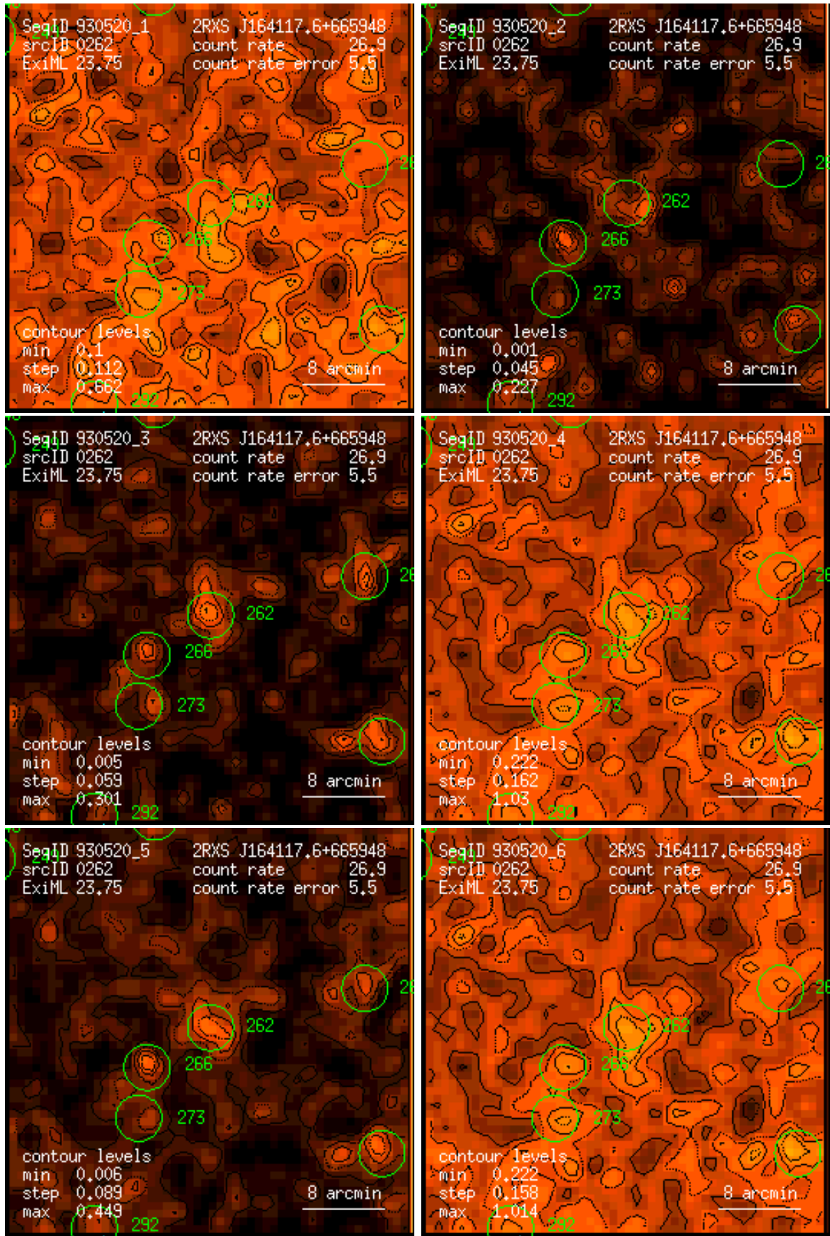
Figure 262: RASS 930520: detection 0262: band rate images, Gaussian filter: (1) PSPC channels 11 – 41, (2) 52 – 90, (3) 91 – 201, (4) 11 – 235, (5) 52 – 201, (6) 11 – 201. Broad band rates in counts/ks. Band rate contour levels in counts/ks/arcmin 2 .
