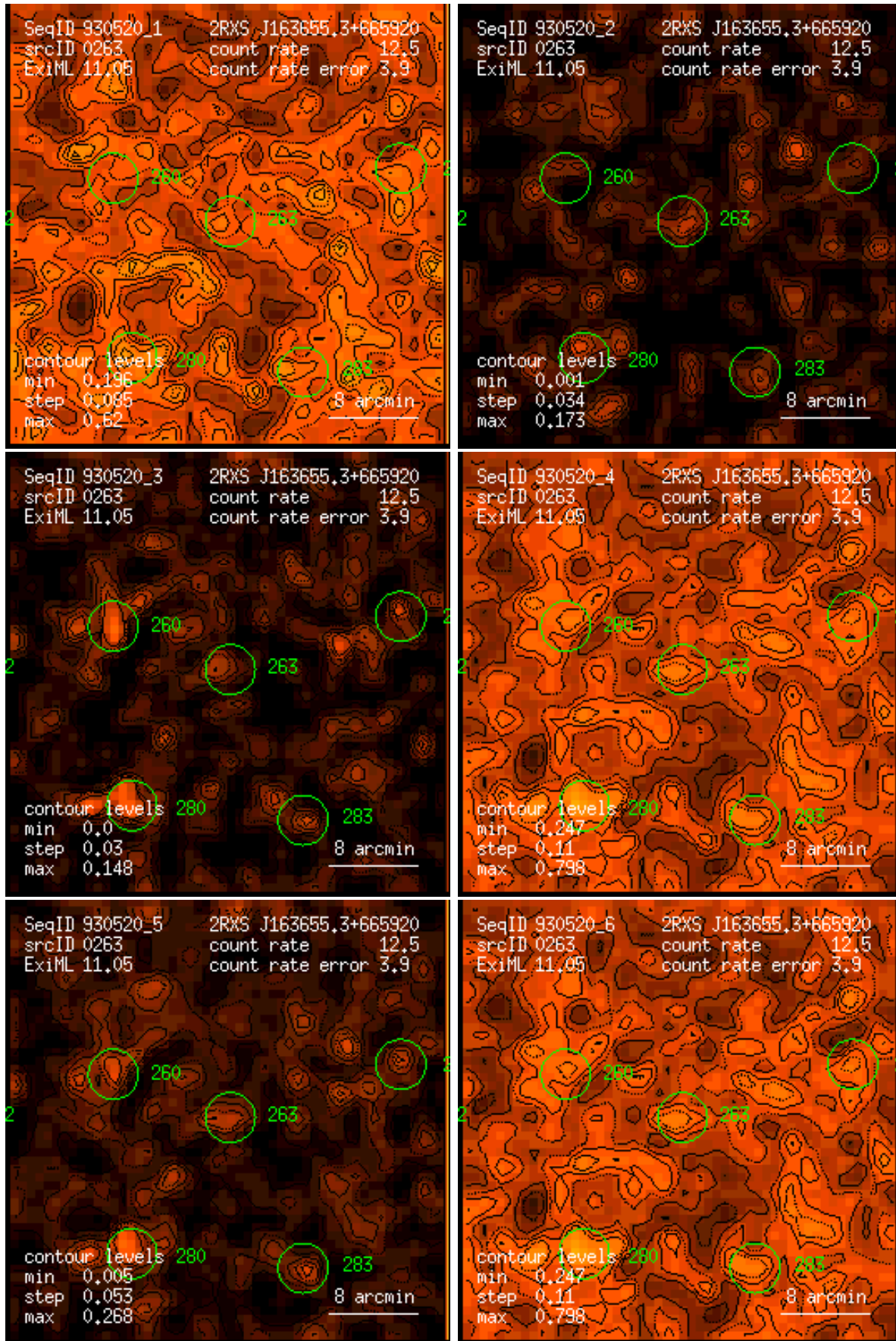
Figure 263: RASS 930520: detection 0263: band rate images, Gaussian filter: (1) PSPC channels 11 – 41, (2) 52 – 90, (3) 91 – 201, (4) 11 – 235, (5) 52 – 201, (6) 11 – 201. Broad band rates in counts/ks. Band rate contour levels in counts/ks/arcmin 2 .
