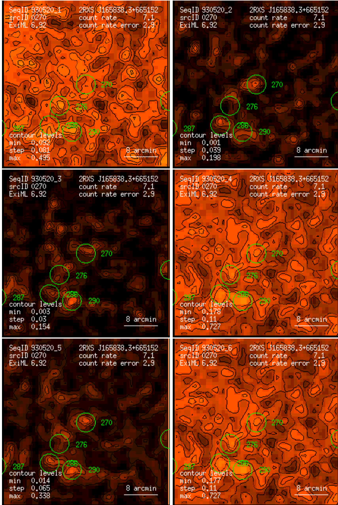
Figure 270: RASS 930520: detection 0270: band rate images, Gaussian filter: (1) PSPC channels 11 – 41, (2) 52 – 90, (3) 91 – 201, (4) 11 – 235, (5) 52 – 201, (6) 11 – 201. Broad band rates in counts/ks. Band rate contour levels in counts/ks/arcmin 2 .
