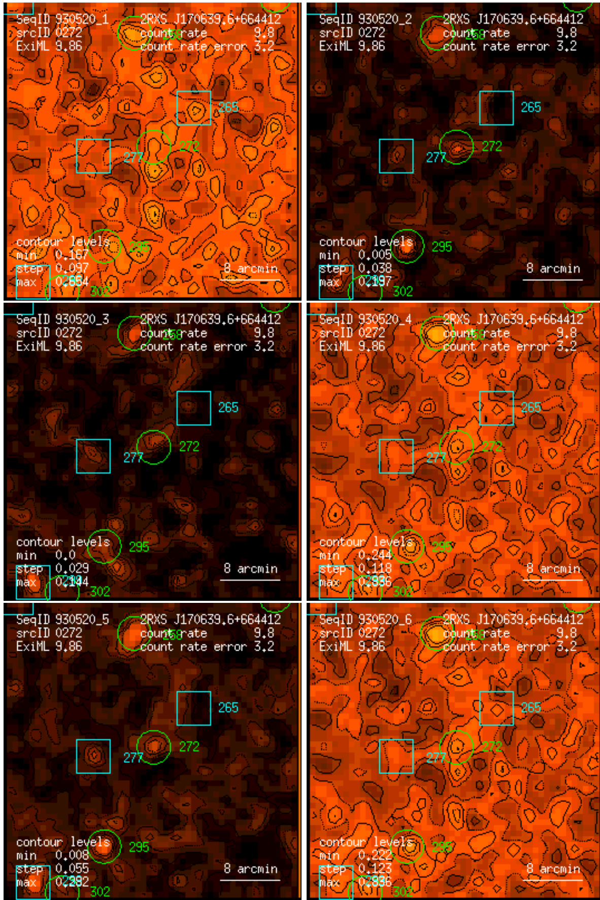
Figure 272: RASS 930520: detection 0272: band rate images, Gaussian filter: (1) PSPC channels 11 – 41, (2) 52 – 90, (3) 91 – 201, (4) 11 – 235, (5) 52 – 201, (6) 11 – 201. Broad band rates in counts/ks. Band rate contour levels in counts/ks/arcmin 2 .
