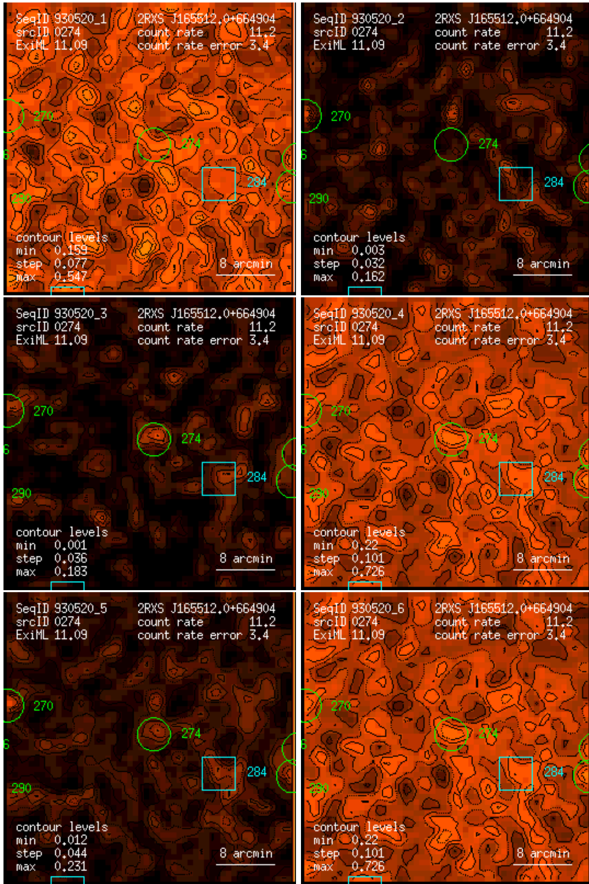
Figure 274: RASS 930520: detection 0274: band rate images, Gaussian filter: (1) PSPC channels 11 – 41, (2) 52 – 90, (3) 91 – 201, (4) 11 – 235, (5) 52 – 201, (6) 11 – 201. Broad band rates in counts/ks. Band rate contour levels in counts/ks/arcmin 2 .
