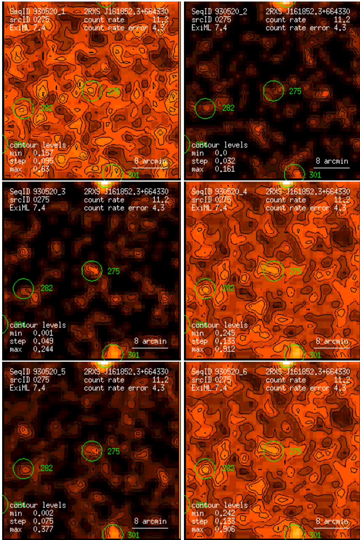
Figure 275: RASS 930520: detection 0275: band rate images, Gaussian filter: (1) PSPC channels 11 – 41, (2) 52 – 90, (3) 91 – 201, (4) 11 – 235, (5) 52 – 201, (6) 11 – 201. Broad band rates in counts/ks. Band rate contour levels in counts/ks/arcmin 2 .
