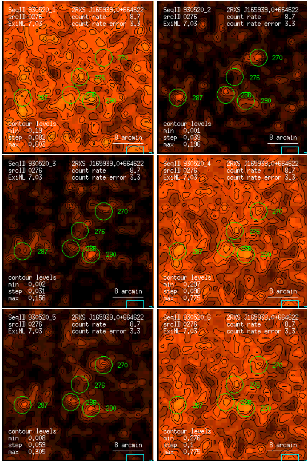
Figure 276: RASS 930520: detection 0276: band rate images, Gaussian filter: (1) PSPC channels 11 – 41, (2) 52 – 90, (3) 91 – 201, (4) 11 – 235, (5) 52 – 201, (6) 11 – 201. Broad band rates in counts/ks. Band rate contour levels in counts/ks/arcmin 2 .
