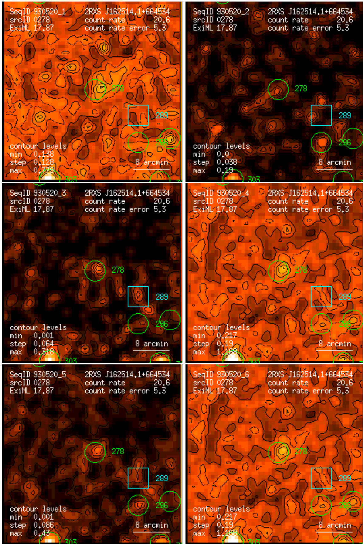
Figure 278: RASS 930520: detection 0278: band rate images, Gaussian filter: (1) PSPC channels 11 – 41, (2) 52 – 90, (3) 91 – 201, (4) 11 – 235, (5) 52 – 201, (6) 11 – 201. Broad band rates in counts/ks. Band rate contour levels in counts/ks/arcmin 2 .
