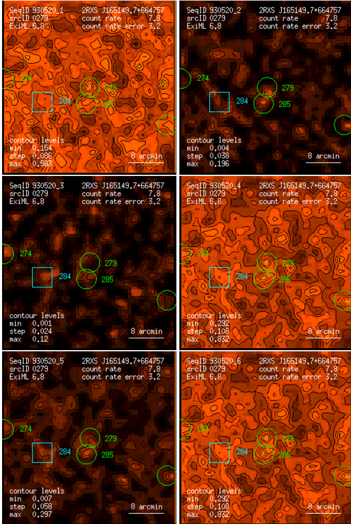
Figure 279: RASS 930520: detection 0279: band rate images, Gaussian filter: (1) PSPC channels 11 – 41, (2) 52 – 90, (3) 91 – 201, (4) 11 – 235, (5) 52 – 201, (6) 11 – 201. Broad band rates in counts/ks. Band rate contour levels in counts/ks/arcmin 2 .
