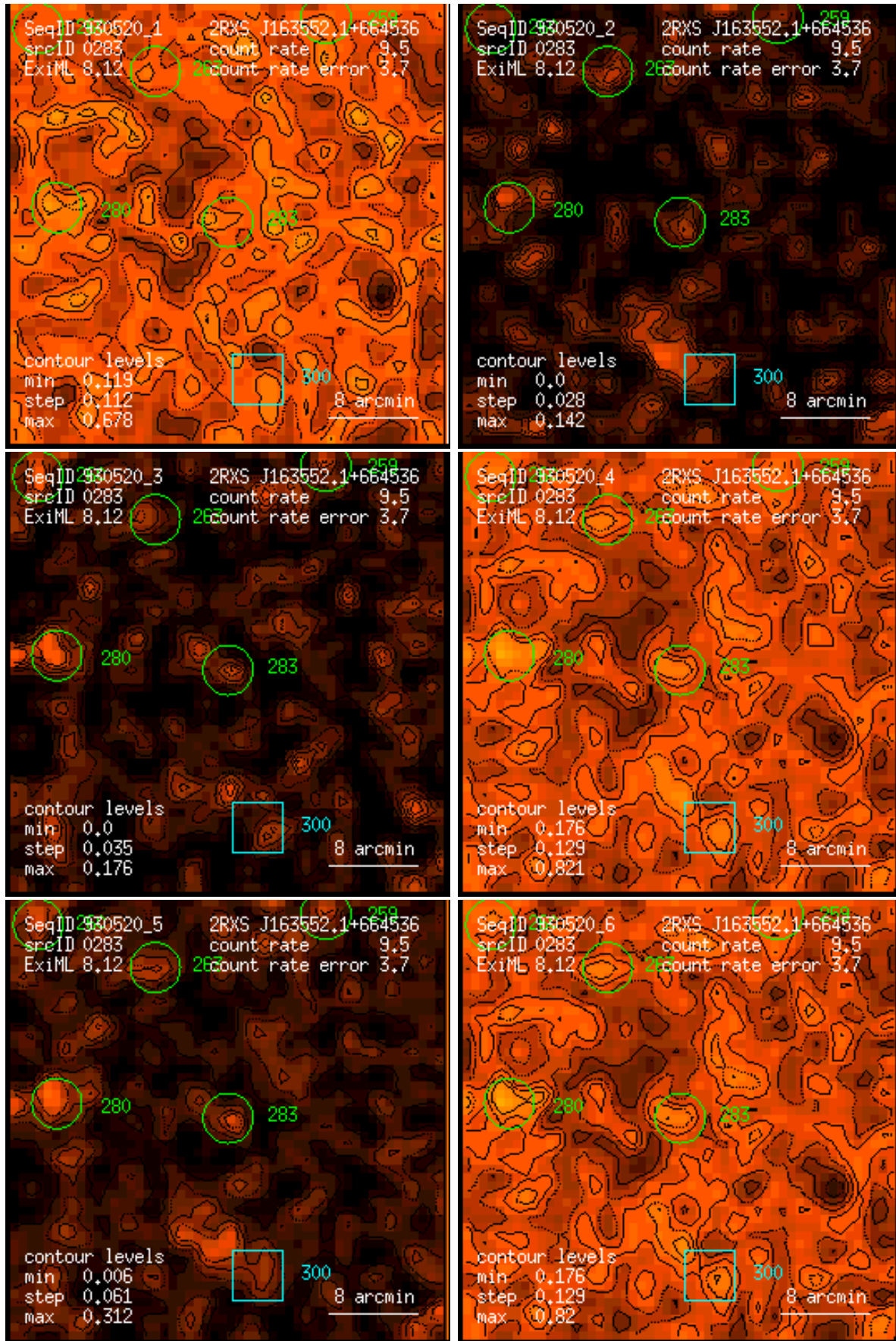
Figure 283: RASS 930520: detection 0283: band rate images, Gaussian filter: (1) PSPC channels 11 – 41, (2) 52 – 90, (3) 91 – 201, (4) 11 – 235, (5) 52 – 201, (6) 11 – 201. Broad band rates in counts/ks. Band rate contour levels in counts/ks/arcmin 2 .
