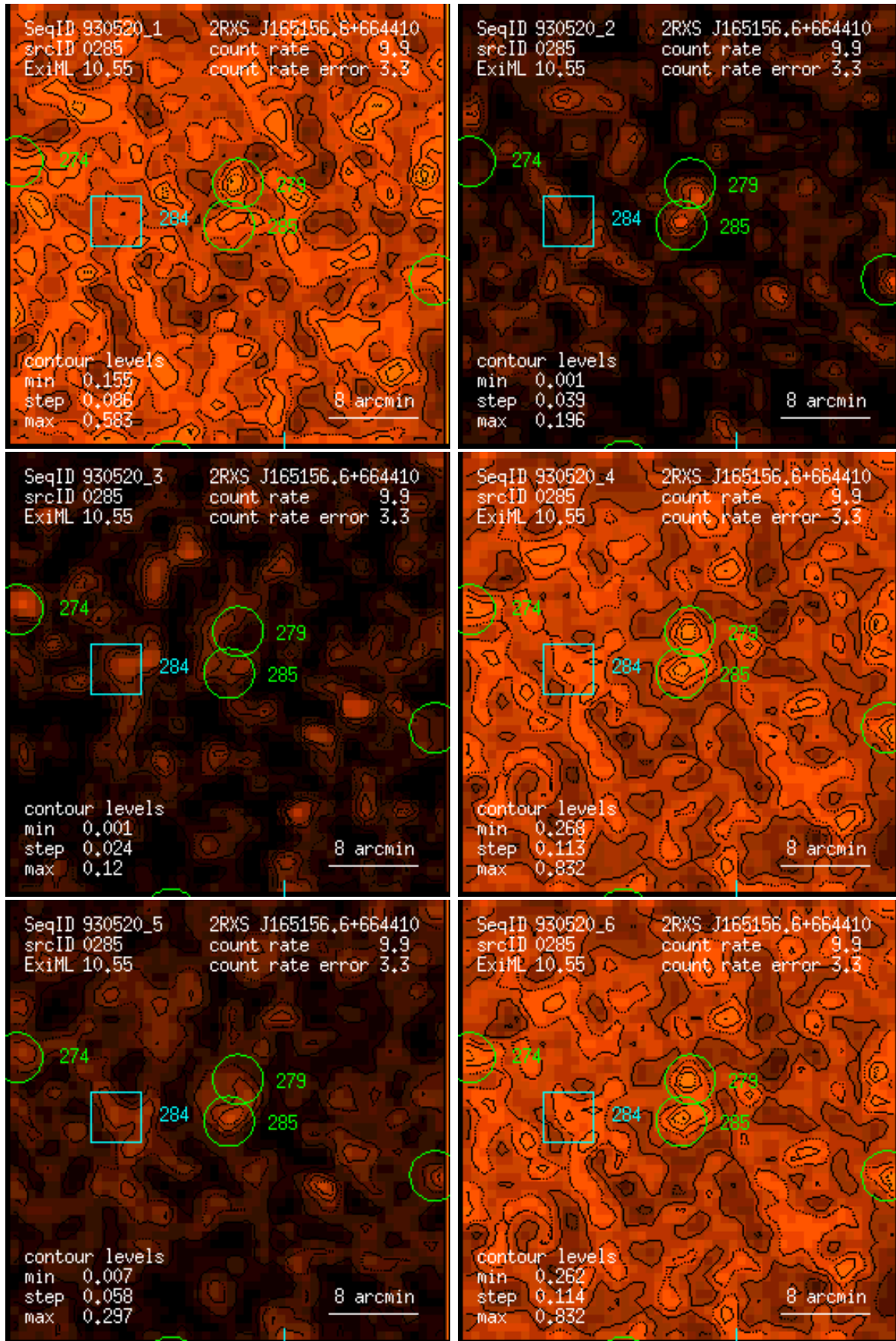
Figure 285: RASS 930520: detection 0285: band rate images, Gaussian filter: (1) PSPC channels 11 – 41, (2) 52 – 90, (3) 91 – 201, (4) 11 – 235, (5) 52 – 201, (6) 11 – 201. Broad band rates in counts/ks. Band rate contour levels in counts/ks/arcmin 2 .
