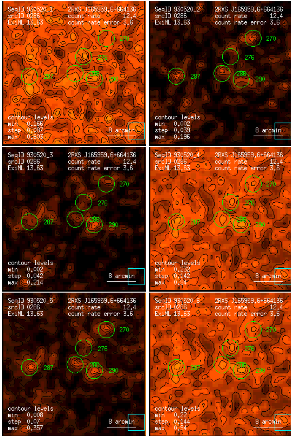
Figure 286: RASS 930520: detection 0286: band rate images, Gaussian filter: (1) PSPC channels 11 – 41, (2) 52 – 90, (3) 91 – 201, (4) 11 – 235, (5) 52 – 201, (6) 11 – 201. Broad band rates in counts/ks. Band rate contour levels in counts/ks/arcmin 2 .
