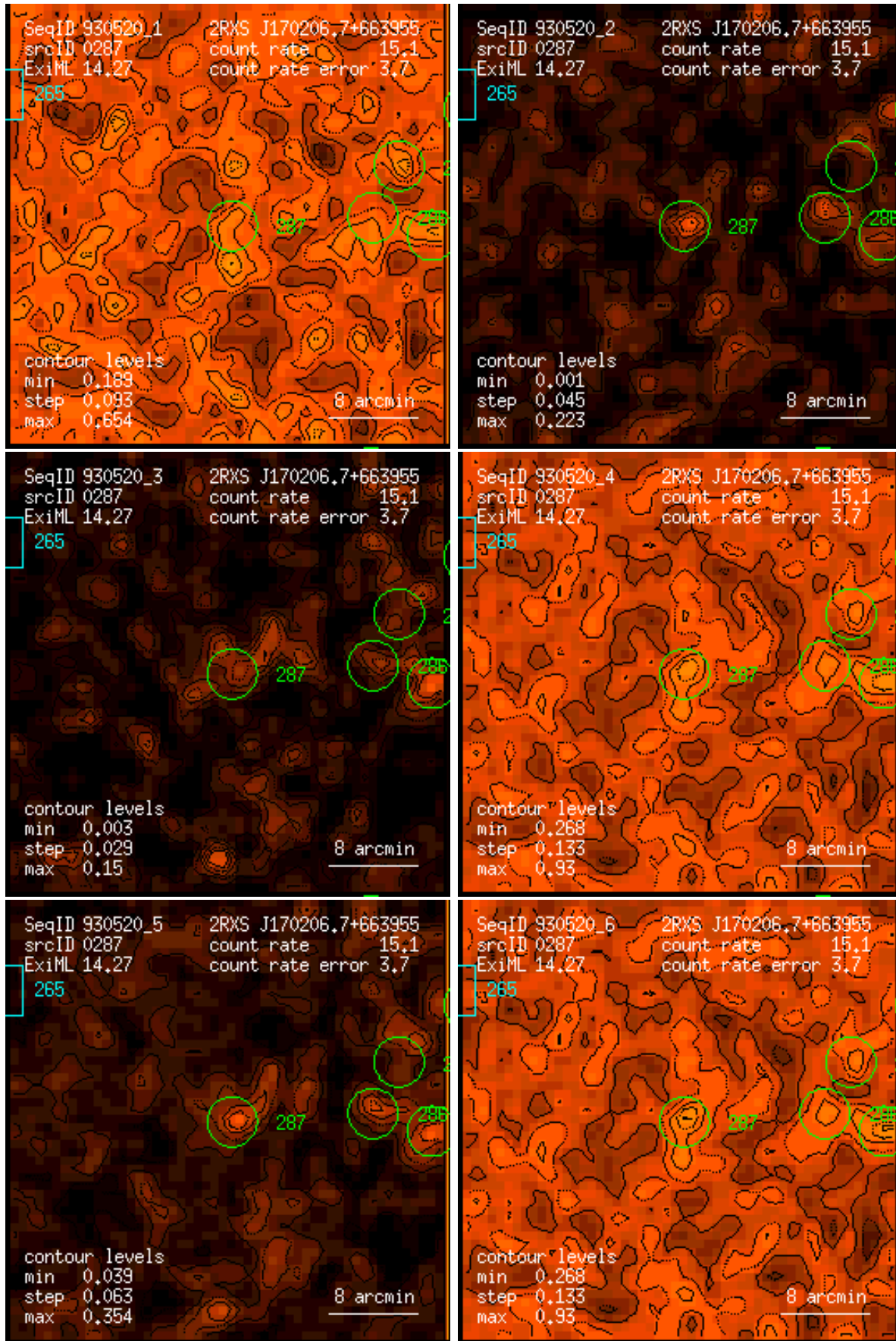
Figure 287: RASS 930520: detection 0287: band rate images, Gaussian filter: (1) PSPC channels 11 – 41, (2) 52 – 90, (3) 91 – 201, (4) 11 – 235, (5) 52 – 201, (6) 11 – 201. Broad band rates in counts/ks. Band rate contour levels in counts/ks/arcmin 2 .
