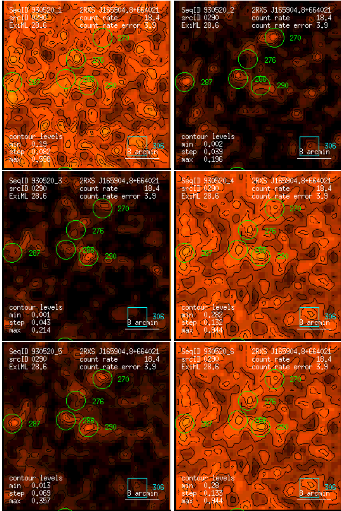
Figure 290: RASS 930520: detection 0290: band rate images, Gaussian filter: (1) PSPC channels 11 – 41, (2) 52 – 90, (3) 91 – 201, (4) 11 – 235, (5) 52 – 201, (6) 11 – 201. Broad band rates in counts/ks. Band rate contour levels in counts/ks/arcmin 2 .
