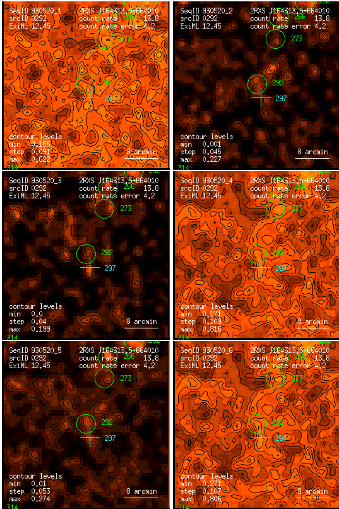
Figure 292: RASS 930520: detection 0292: band rate images, Gaussian filter: (1) PSPC channels 11 – 41, (2) 52 – 90, (3) 91 – 201, (4) 11 – 235, (5) 52 – 201, (6) 11 – 201. Broad band rates in counts/ks. Band rate contour levels in counts/ks/arcmin 2 .
