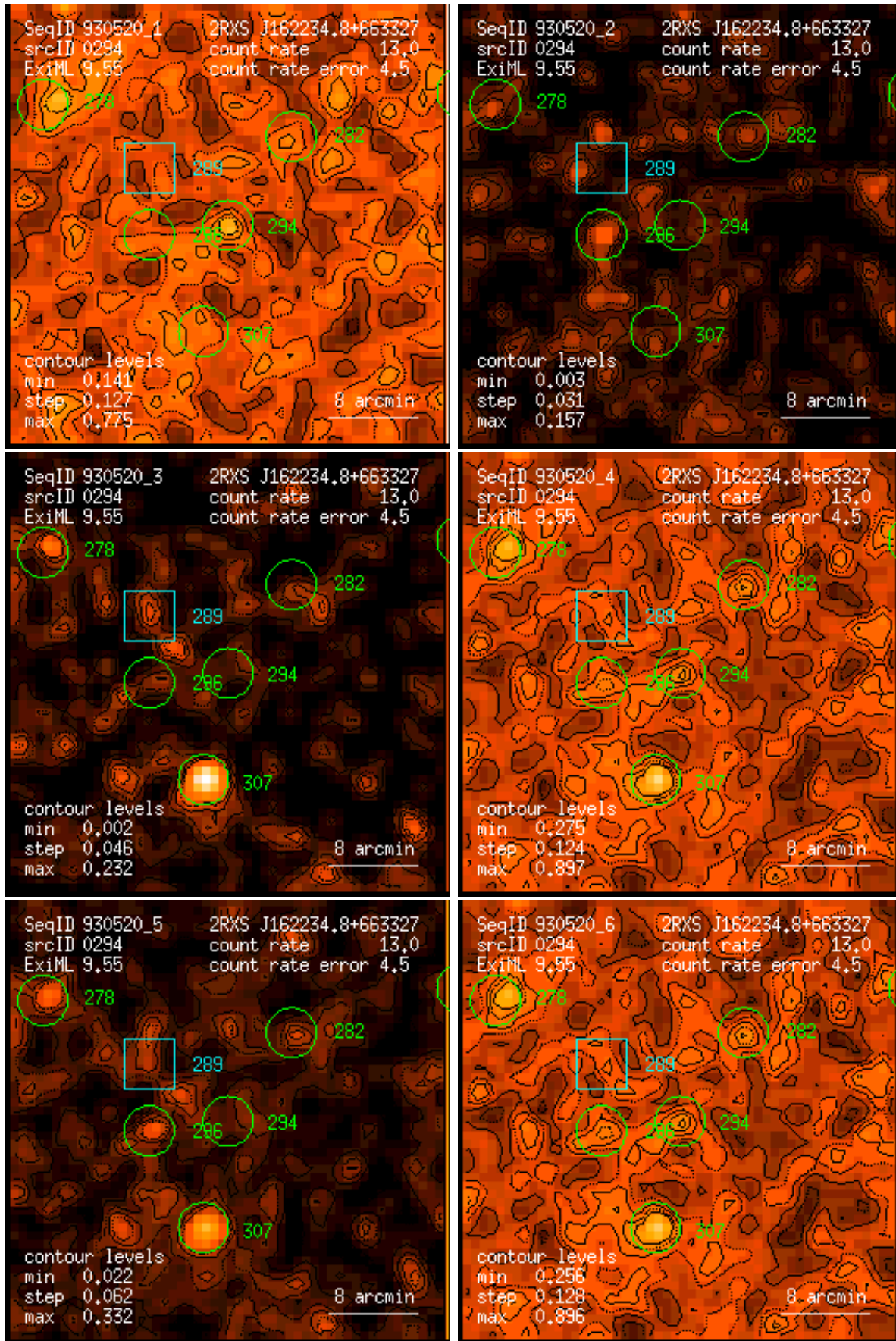
Figure 294: RASS 930520: detection 0294: band rate images, Gaussian filter: (1) PSPC channels 11 – 41, (2) 52 – 90, (3) 91 – 201, (4) 11 – 235, (5) 52 – 201, (6) 11 – 201. Broad band rates in counts/ks. Band rate contour levels in counts/ks/arcmin 2 .
