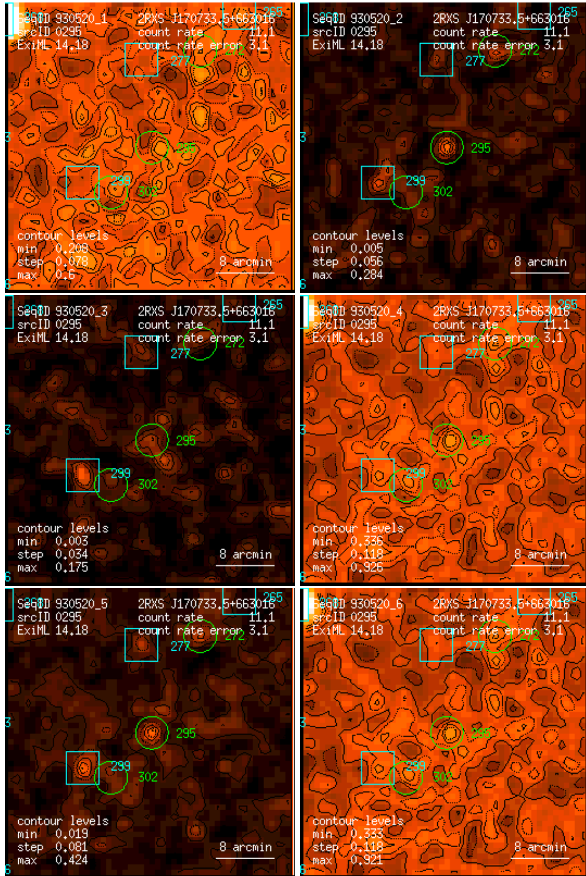
Figure 295: RASS 930520: detection 0295: band rate images, Gaussian filter: (1) PSPC channels 11 – 41, (2) 52 – 90, (3) 91 – 201, (4) 11 – 235, (5) 52 – 201, (6) 11 – 201. Broad band rates in counts/ks. Band rate contour levels in counts/ks/arcmin 2 .
