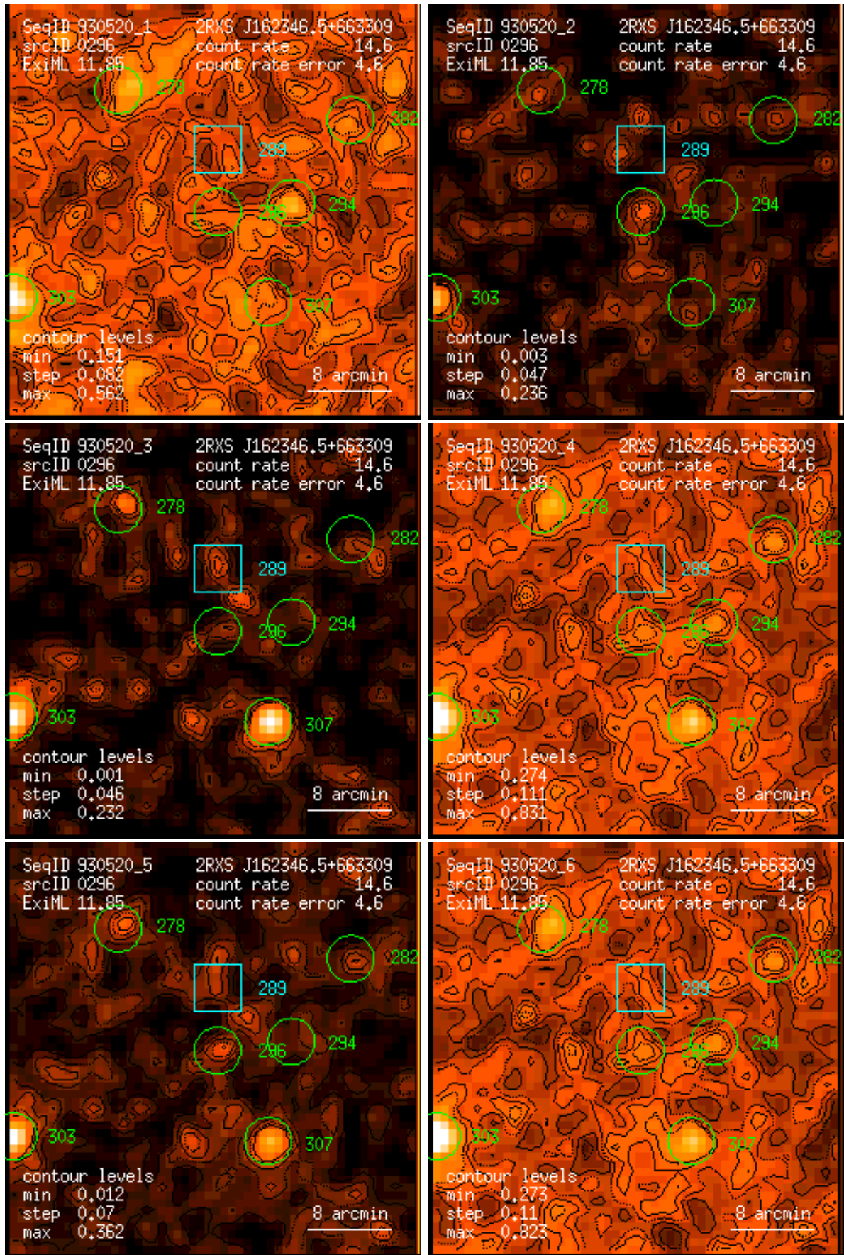
Figure 296: RASS 930520: detection 0296: band rate images, Gaussian filter: (1) PSPC channels 11 – 41, (2) 52 – 90, (3) 91 – 201, (4) 11 – 235, (5) 52 – 201, (6) 11 – 201. Broad band rates in counts/ks. Band rate contour levels in counts/ks/arcmin 2 .
