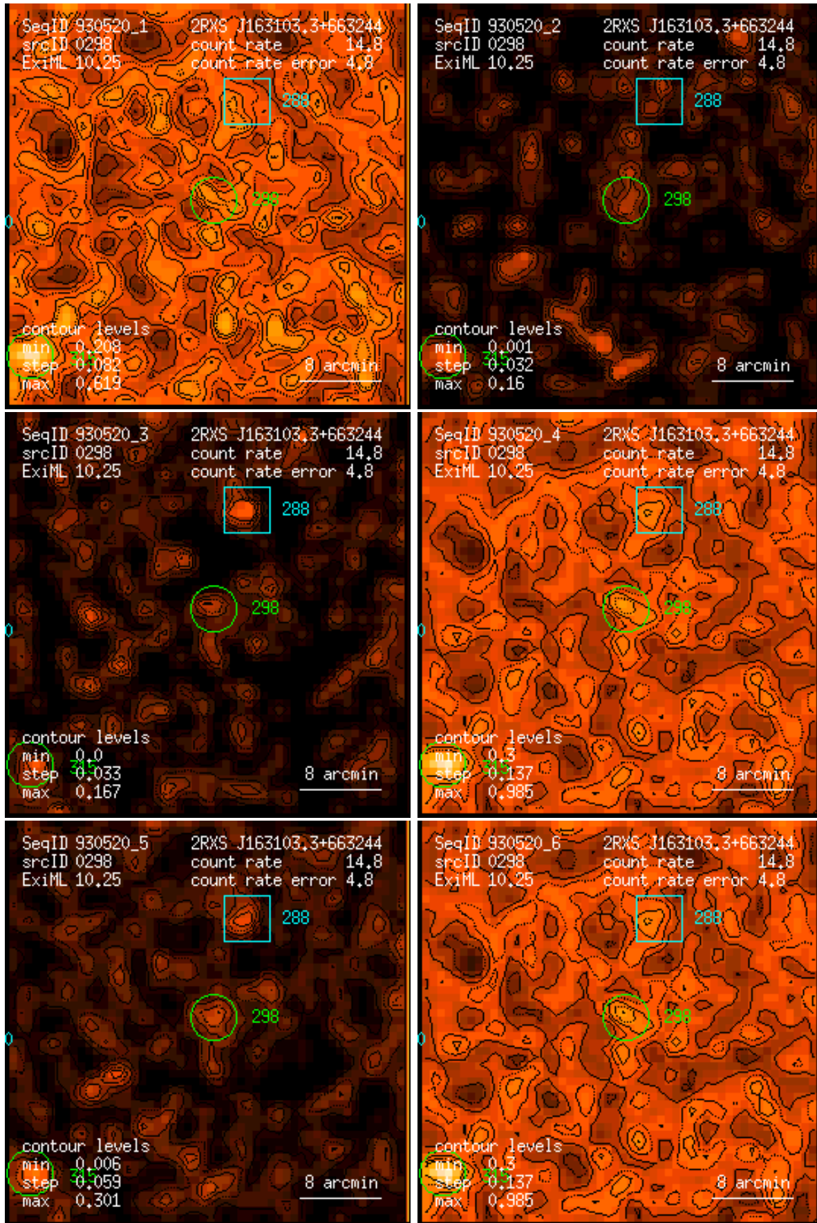
Figure 298: RASS 930520: detection 0298: band rate images, Gaussian filter: (1) PSPC channels 11 – 41, (2) 52 – 90, (3) 91 – 201, (4) 11 – 235, (5) 52 – 201, (6) 11 – 201. Broad band rates in counts/ks. Band rate contour levels in counts/ks/arcmin 2 .
