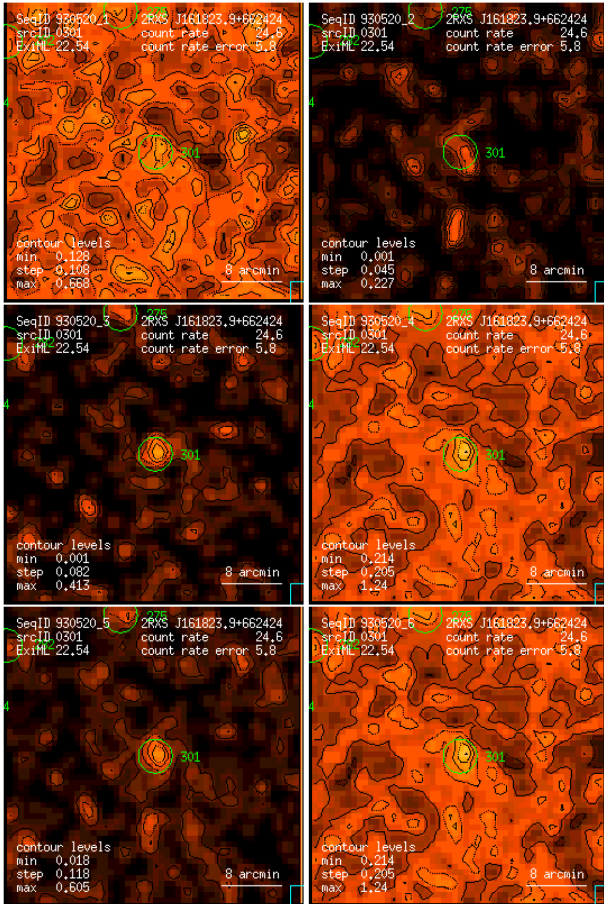
Figure 301: RASS 930520: detection 0301: band rate images, Gaussian filter: (1) PSPC channels 11 – 41, (2) 52 – 90, (3) 91 – 201, (4) 11 – 235, (5) 52 – 201, (6) 11 – 201. Broad band rates in counts/ks. Band rate contour levels in counts/ks/arcmin 2 .
