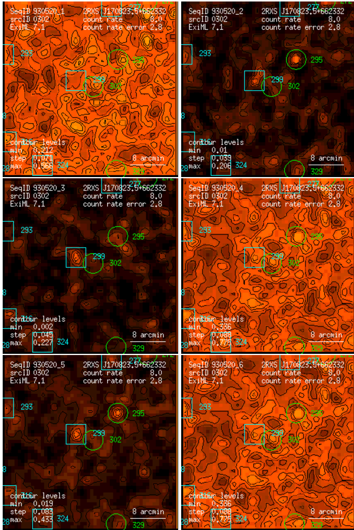
Figure 302: RASS 930520: detection 0302: band rate images, Gaussian filter: (1) PSPC channels 11 – 41, (2) 52 – 90, (3) 91 – 201, (4) 11 – 235, (5) 52 – 201, (6) 11 – 201. Broad band rates in counts/ks. Band rate contour levels in counts/ks/arcmin 2 .
