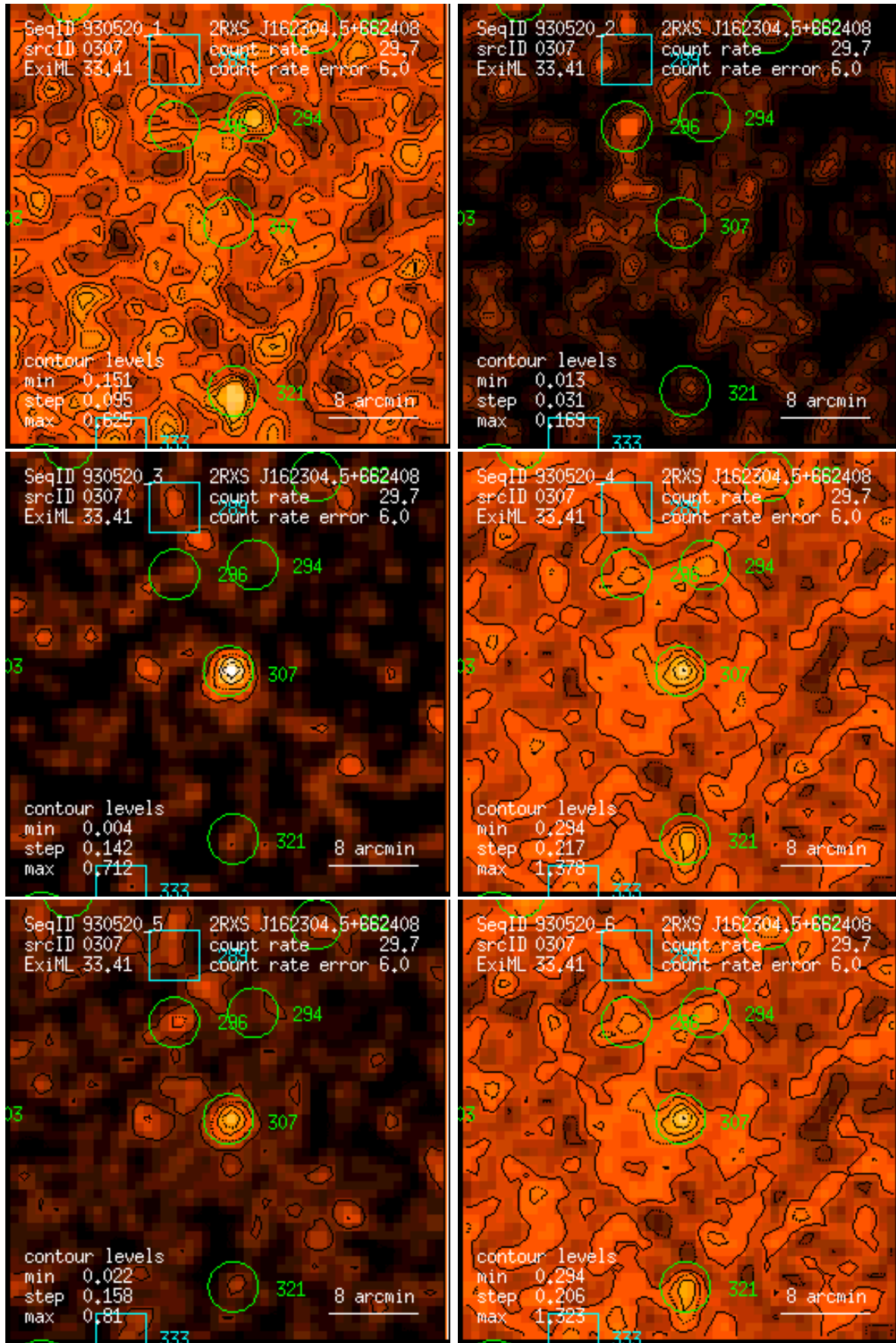
Figure 307: RASS 930520: detection 0307: band rate images, Gaussian filter: (1) PSPC channels 11 – 41, (2) 52 – 90, (3) 91 – 201, (4) 11 – 235, (5) 52 – 201, (6) 11 – 201. Broad band rates in counts/ks. Band rate contour levels in counts/ks/arcmin 2 .
