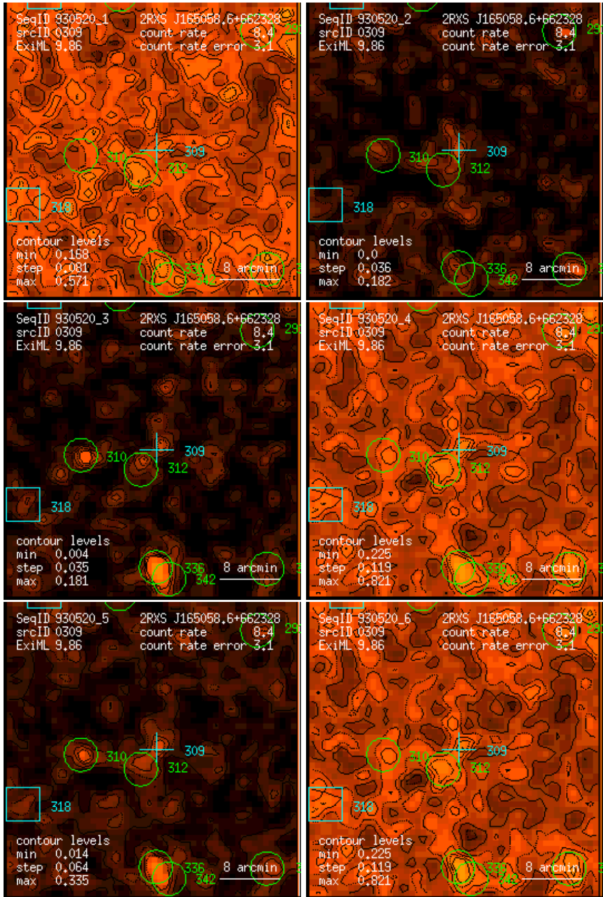
Figure 309: RASS 930520: detection 0309: band rate images, Gaussian filter: (1) PSPC channels 11 – 41, (2) 52 – 90, (3) 91 – 201, (4) 11 – 235, (5) 52 – 201, (6) 11 – 201. Broad band rates in counts/ks. Band rate contour levels in counts/ks/arcmin 2 .
