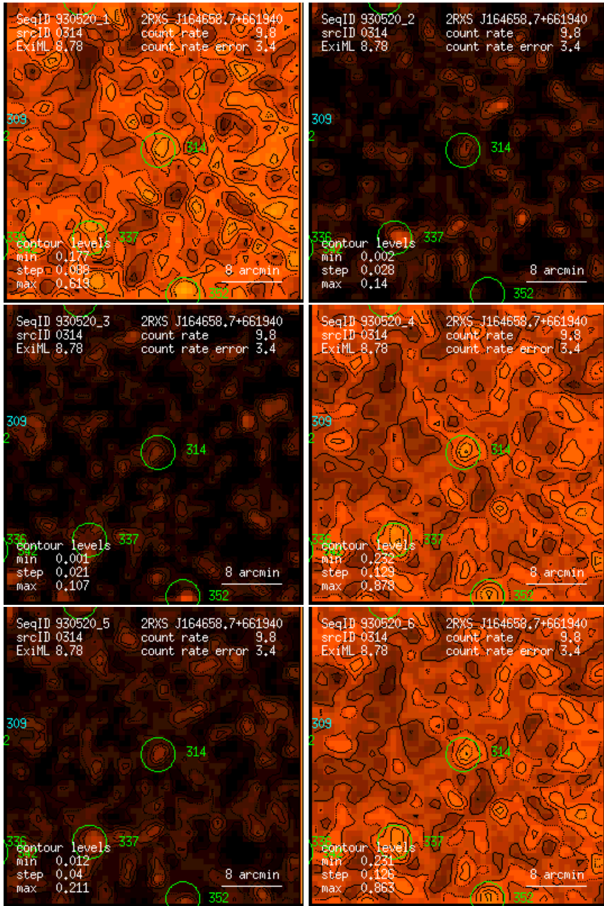
Figure 314: RASS 930520: detection 0314: band rate images, Gaussian filter: (1) PSPC channels 11 – 41, (2) 52 – 90, (3) 91 – 201, (4) 11 – 235, (5) 52 – 201, (6) 11 – 201. Broad band rates in counts/ks. Band rate contour levels in counts/ks/arcmin 2 .
