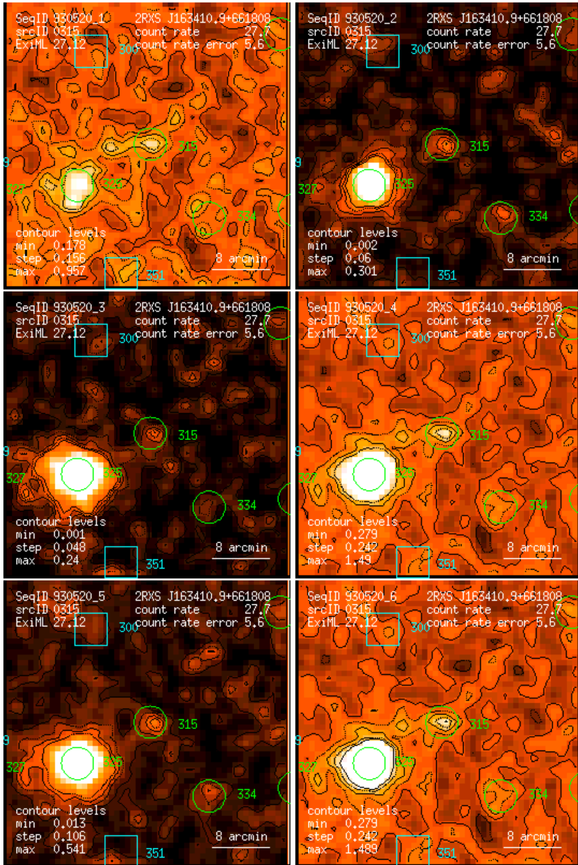
Figure 315: RASS 930520: detection 0315: band rate images, Gaussian filter: (1) PSPC channels 11 – 41, (2) 52 – 90, (3) 91 – 201, (4) 11 – 235, (5) 52 – 201, (6) 11 – 201. Broad band rates in counts/ks. Band rate contour levels in counts/ks/arcmin 2 .
