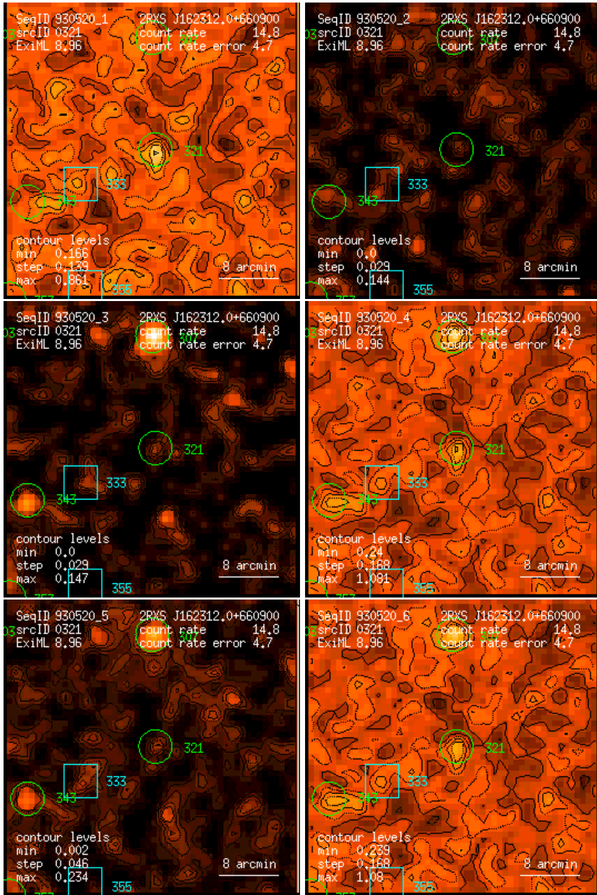
Figure 321: RASS 930520: detection 0321: band rate images, Gaussian filter: (1) PSPC channels 11 – 41, (2) 52 – 90, (3) 91 – 201, (4) 11 – 235, (5) 52 – 201, (6) 11 – 201. Broad band rates in counts/ks. Band rate contour levels in counts/ks/arcmin 2 .
