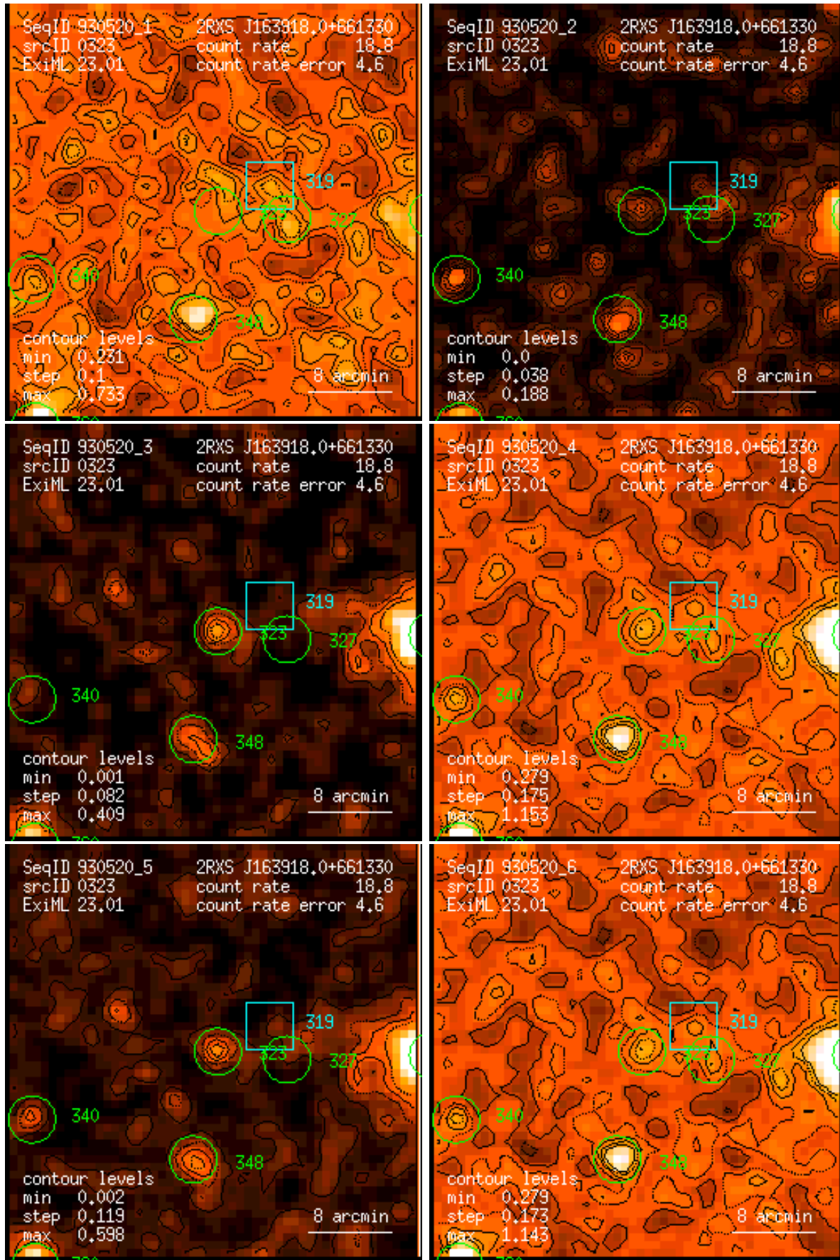
Figure 323: RASS 930520: detection 0323: band rate images, Gaussian filter: (1) PSPC channels 11 – 41, (2) 52 – 90, (3) 91 – 201, (4) 11 – 235, (5) 52 – 201, (6) 11 – 201. Broad band rates in counts/ks. Band rate contour levels in counts/ks/arcmin 2 .
