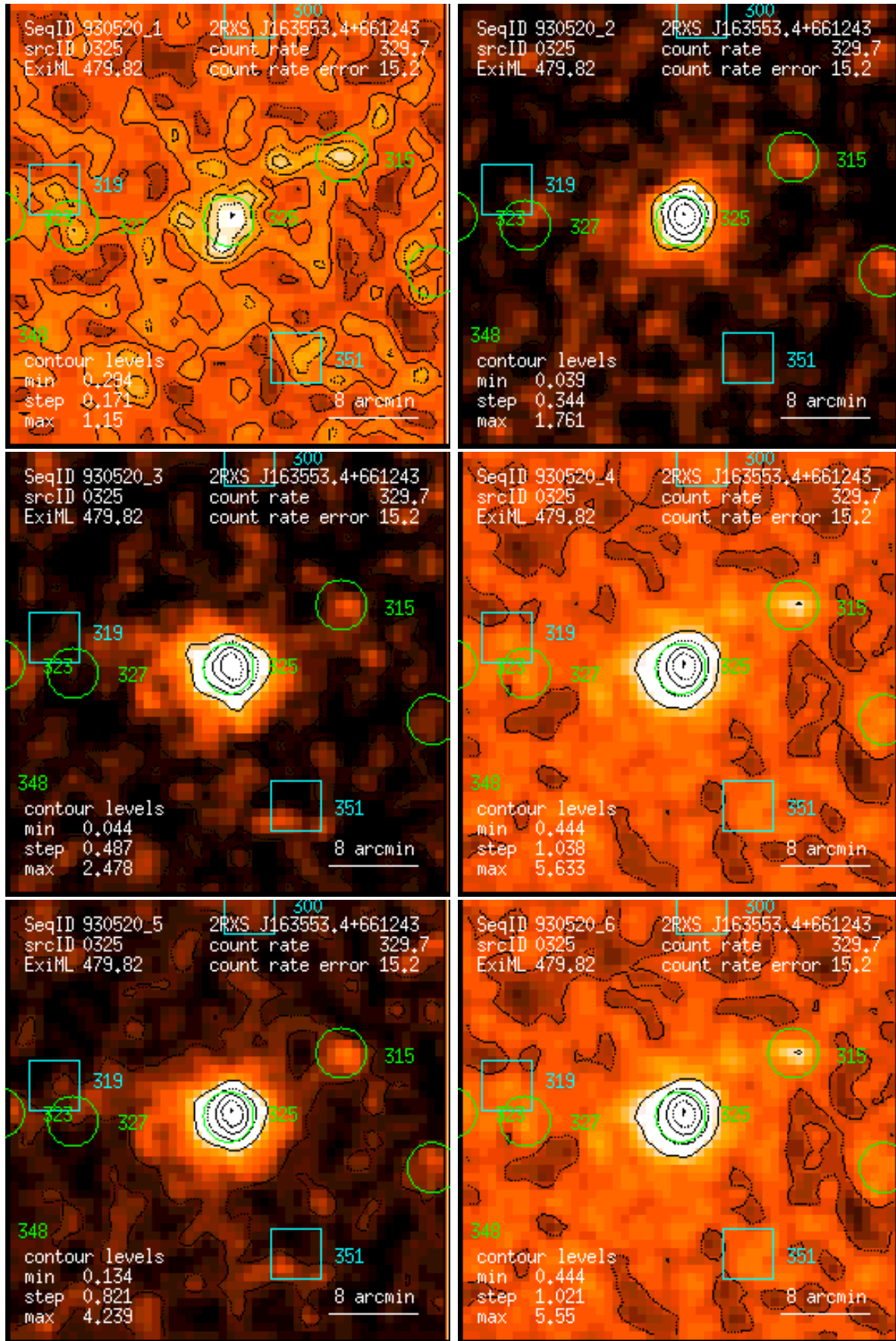
Figure 325: RASS 930520: detection 0325: band rate images, Gaussian filter: (1) PSPC channels 11 – 41, (2) 52 – 90, (3) 91 – 201, (4) 11 – 235, (5) 52 – 201, (6) 11 – 201. Broad band rates in counts/ks. Band rate contour levels in counts/ks/arcmin 2 .
