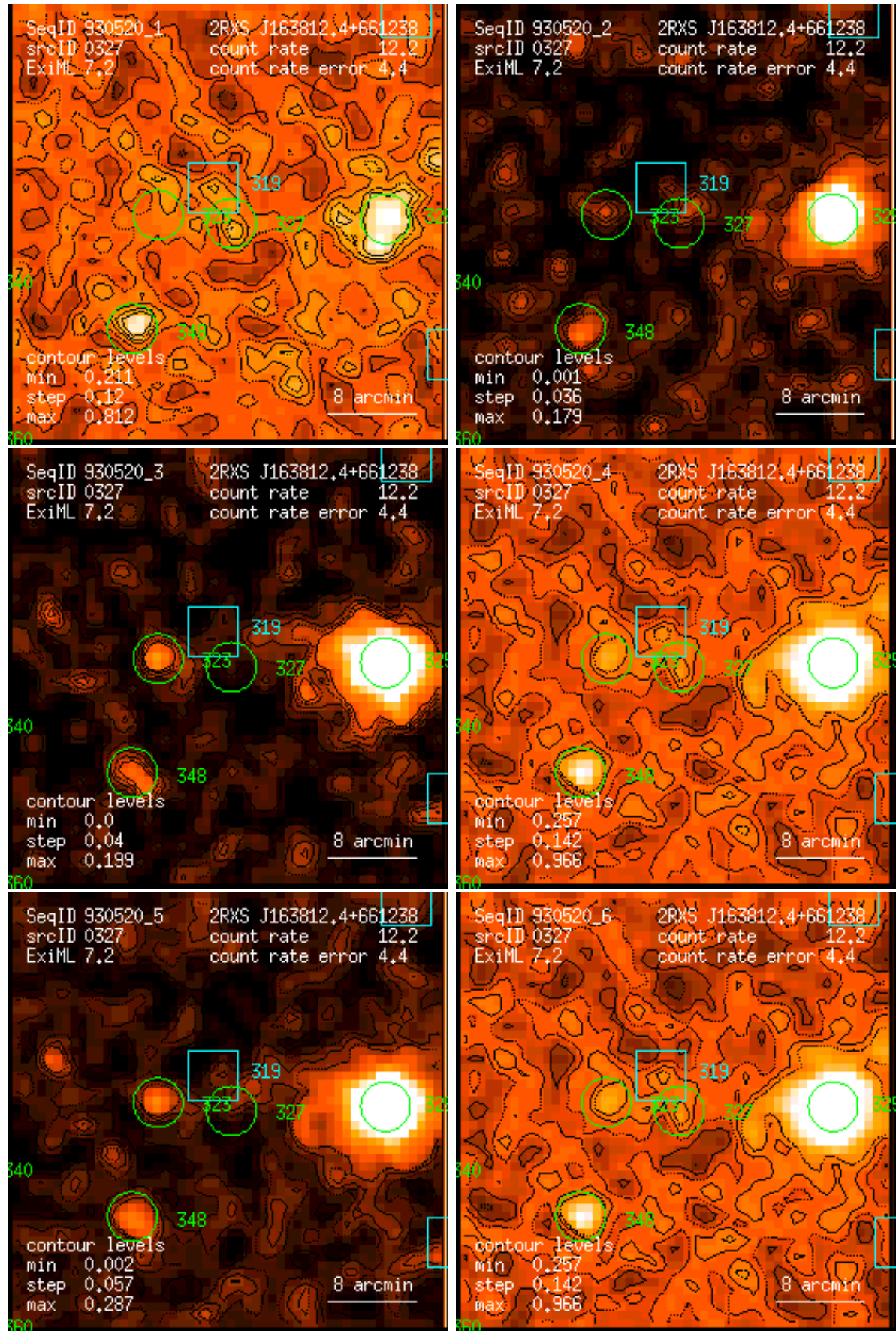
Figure 327: RASS 930520: detection 0327: band rate images, Gaussian filter: (1) PSPC channels 11 – 41, (2) 52 – 90, (3) 91 – 201, (4) 11 – 235, (5) 52 – 201, (6) 11 – 201. Broad band rates in counts/ks. Band rate contour levels in counts/ks/arcmin 2 .
