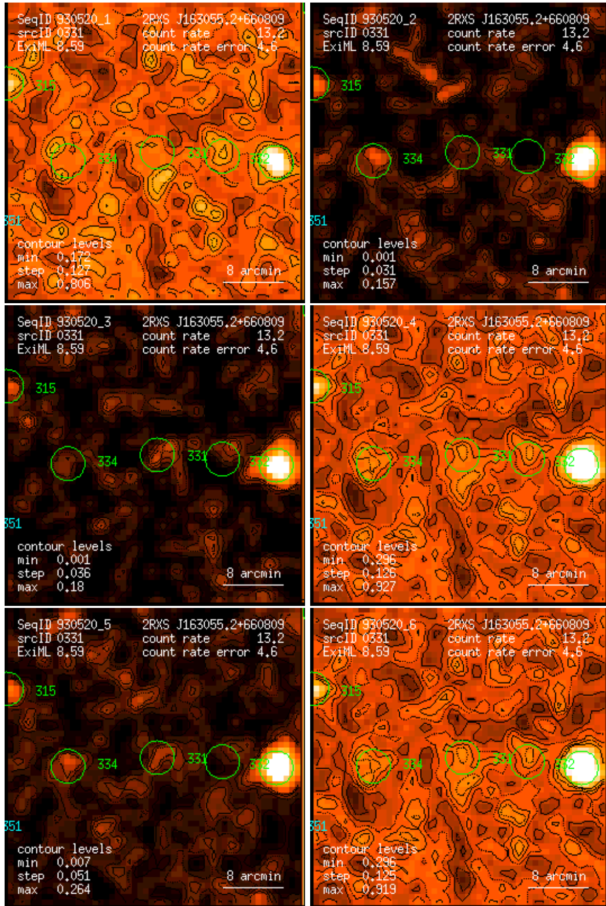
Figure 331: RASS 930520: detection 0331: band rate images, Gaussian filter: (1) PSPC channels 11 – 41, (2) 52 – 90, (3) 91 – 201, (4) 11 – 235, (5) 52 – 201, (6) 11 – 201. Broad band rates in counts/ks. Band rate contour levels in counts/ks/arcmin 2 .
