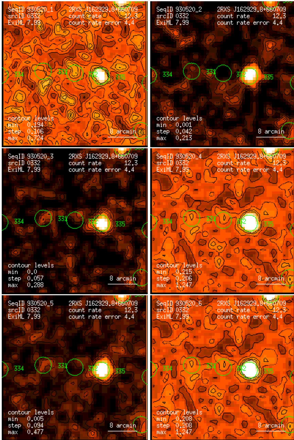
Figure 332: RASS 930520: detection 0332: band rate images, Gaussian filter: (1) PSPC channels 11 – 41, (2) 52 – 90, (3) 91 – 201, (4) 11 – 235, (5) 52 – 201, (6) 11 – 201. Broad band rates in counts/ks. Band rate contour levels in counts/ks/arcmin 2 .
