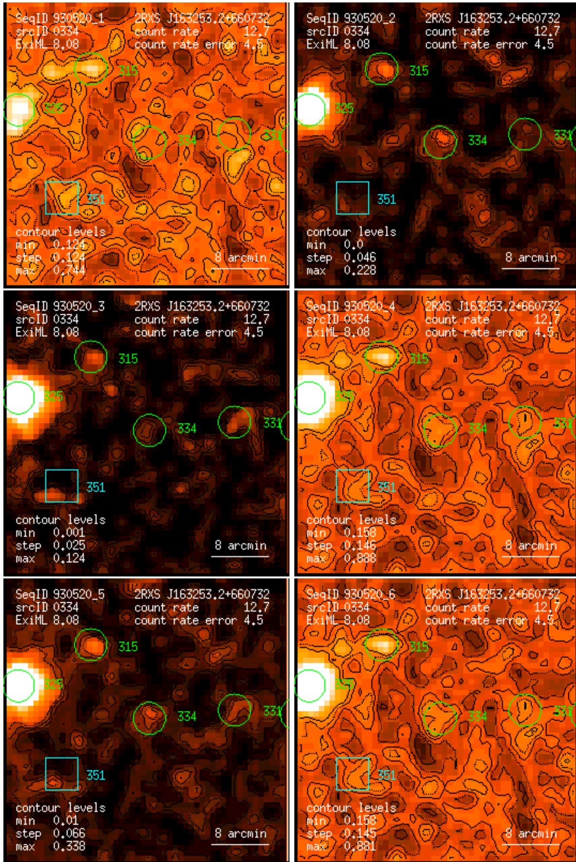
Figure 334: RASS 930520: detection 0334: band rate images, Gaussian filter: (1) PSPC channels 11 – 41, (2) 52 – 90, (3) 91 – 201, (4) 11 – 235, (5) 52 – 201, (6) 11 – 201. Broad band rates in counts/ks. Band rate contour levels in counts/ks/arcmin 2 .
