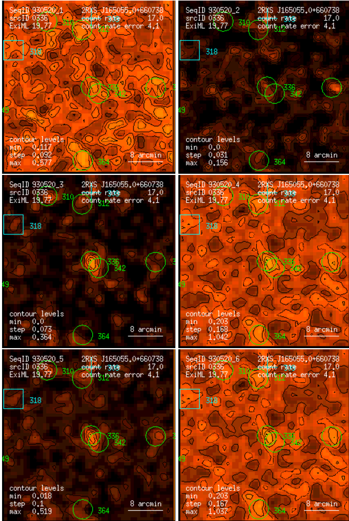
Figure 336: RASS 930520: detection 0336: band rate images, Gaussian filter: (1) PSPC channels 11 – 41, (2) 52 – 90, (3) 91 – 201, (4) 11 – 235, (5) 52 – 201, (6) 11 – 201. Broad band rates in counts/ks. Band rate contour levels in counts/ks/arcmin 2 .
