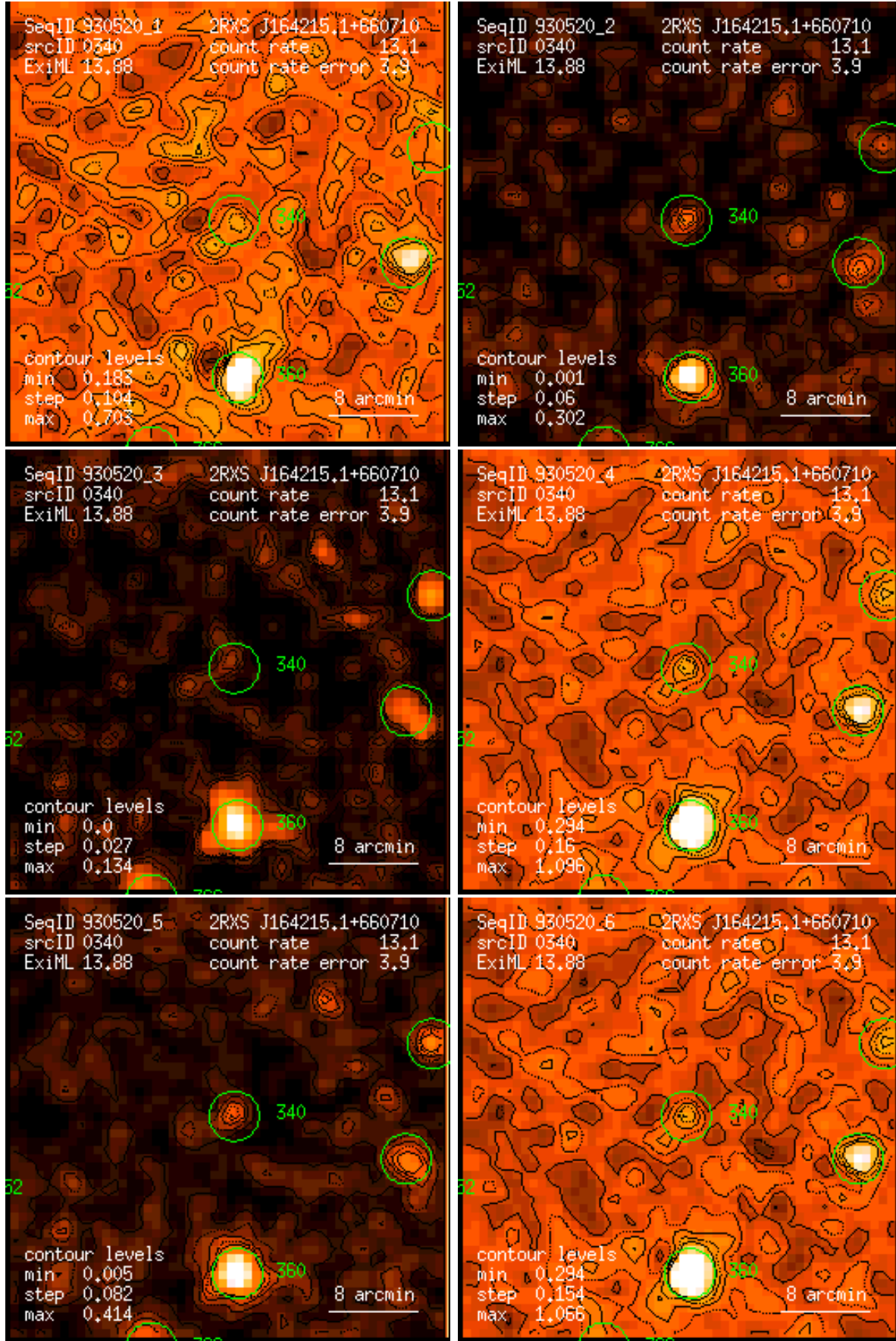
Figure 340: RASS 930520: detection 0340: band rate images, Gaussian filter: (1) PSPC channels 11 – 41, (2) 52 – 90, (3) 91 – 201, (4) 11 – 235, (5) 52 – 201, (6) 11 – 201. Broad band rates in counts/ks. Band rate contour levels in counts/ks/arcmin 2 .
