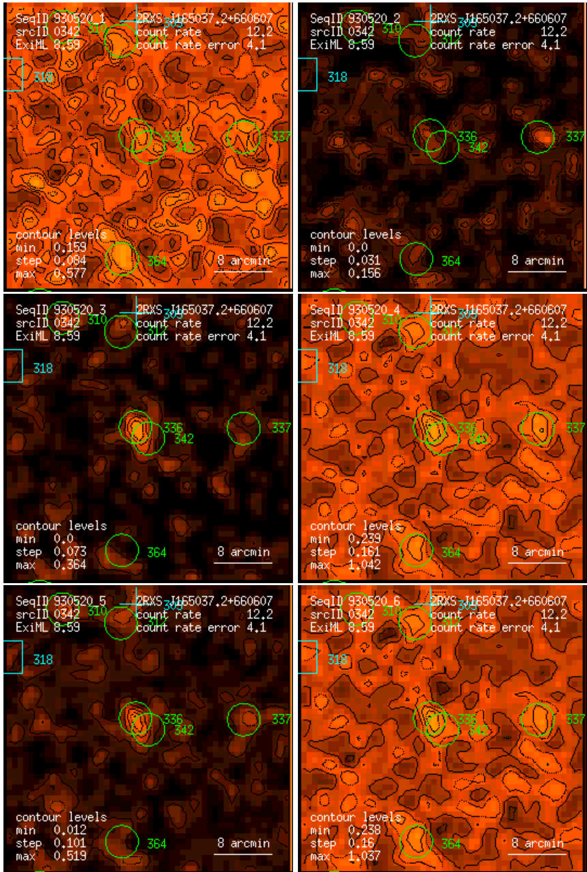
Figure 342: RASS 930520: detection 0342: band rate images, Gaussian filter: (1) PSPC channels 11 – 41, (2) 52 – 90, (3) 91 – 201, (4) 11 – 235, (5) 52 – 201, (6) 11 – 201. Broad band rates in counts/ks. Band rate contour levels in counts/ks/arcmin 2 .
