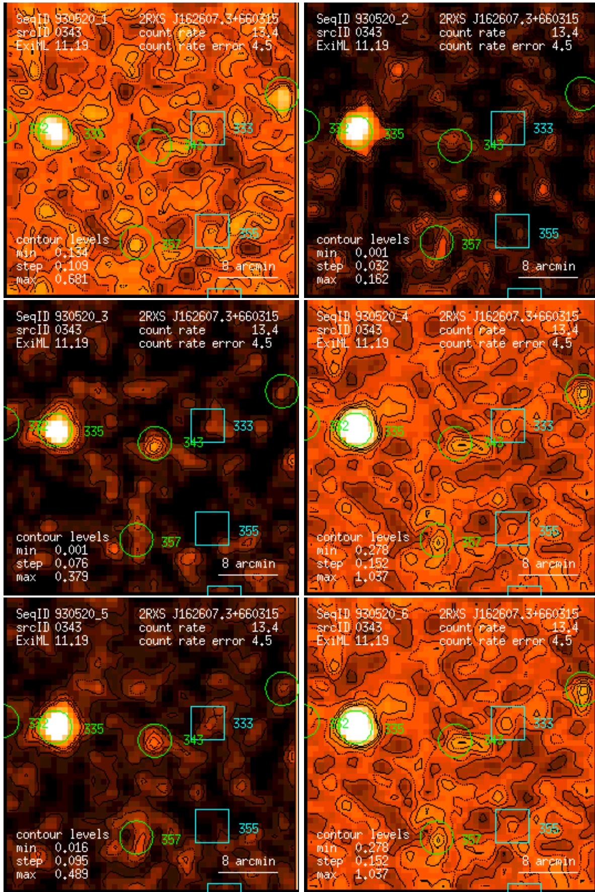
Figure 343: RASS 930520: detection 0343: band rate images, Gaussian filter: (1) PSPC channels 11 – 41, (2) 52 – 90, (3) 91 – 201, (4) 11 – 235, (5) 52 – 201, (6) 11 – 201. Broad band rates in counts/ks. Band rate contour levels in counts/ks/arcmin 2 .
