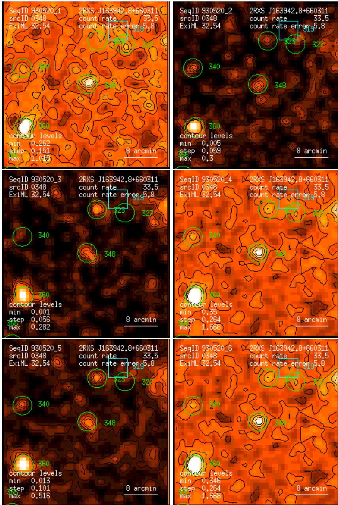
Figure 348: RASS 930520: detection 0348: band rate images, Gaussian filter: (1) PSPC channels 11 – 41, (2) 52 – 90, (3) 91 – 201, (4) 11 – 235, (5) 52 – 201, (6) 11 – 201. Broad band rates in counts/ks. Band rate contour levels in counts/ks/arcmin 2 .
