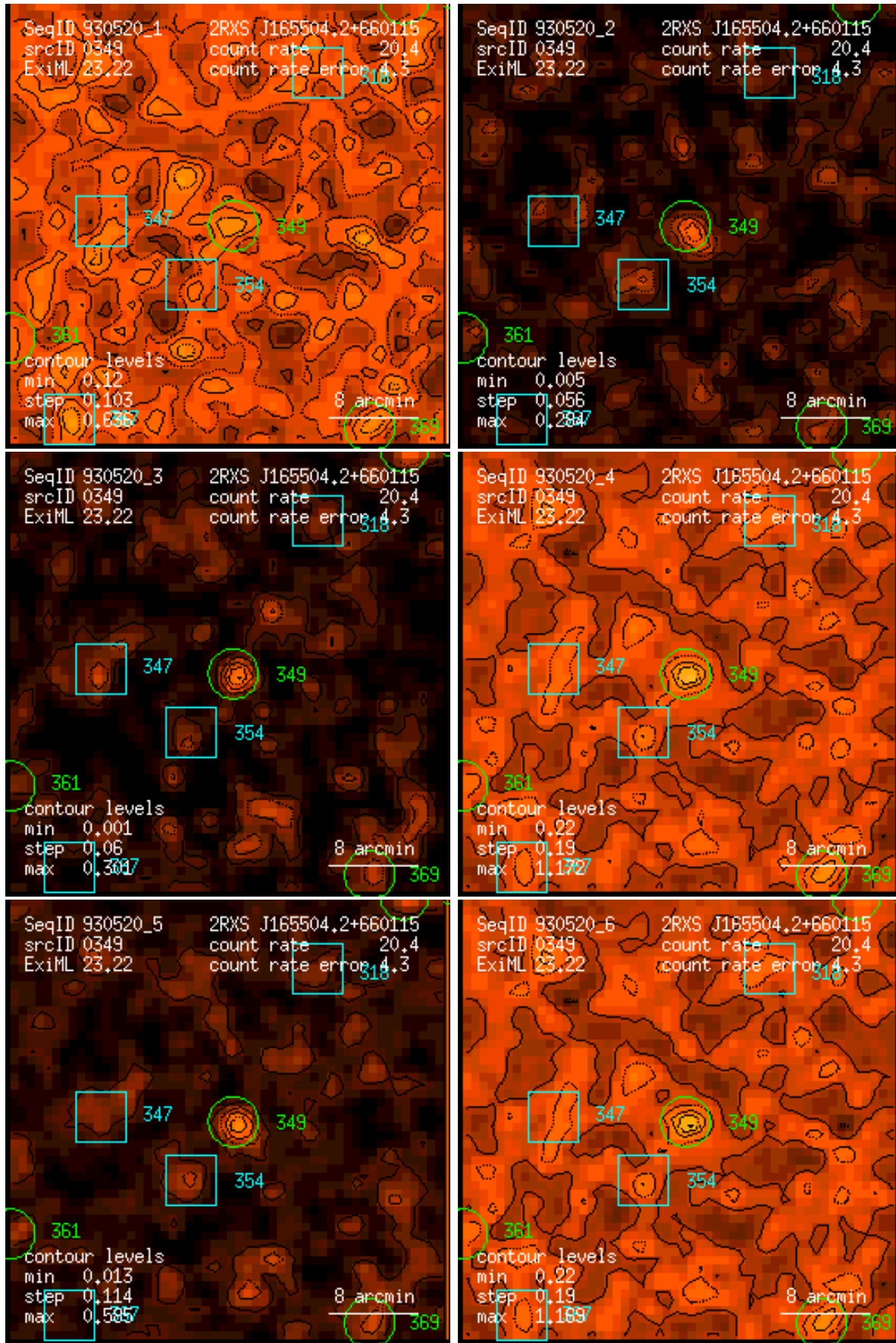
Figure 349: RASS 930520: detection 0349: band rate images, Gaussian filter: (1) PSPC channels 11 – 41, (2) 52 – 90, (3) 91 – 201, (4) 11 – 235, (5) 52 – 201, (6) 11 – 201. Broad band rates in counts/ks. Band rate contour levels in counts/ks/arcmin 2 .
