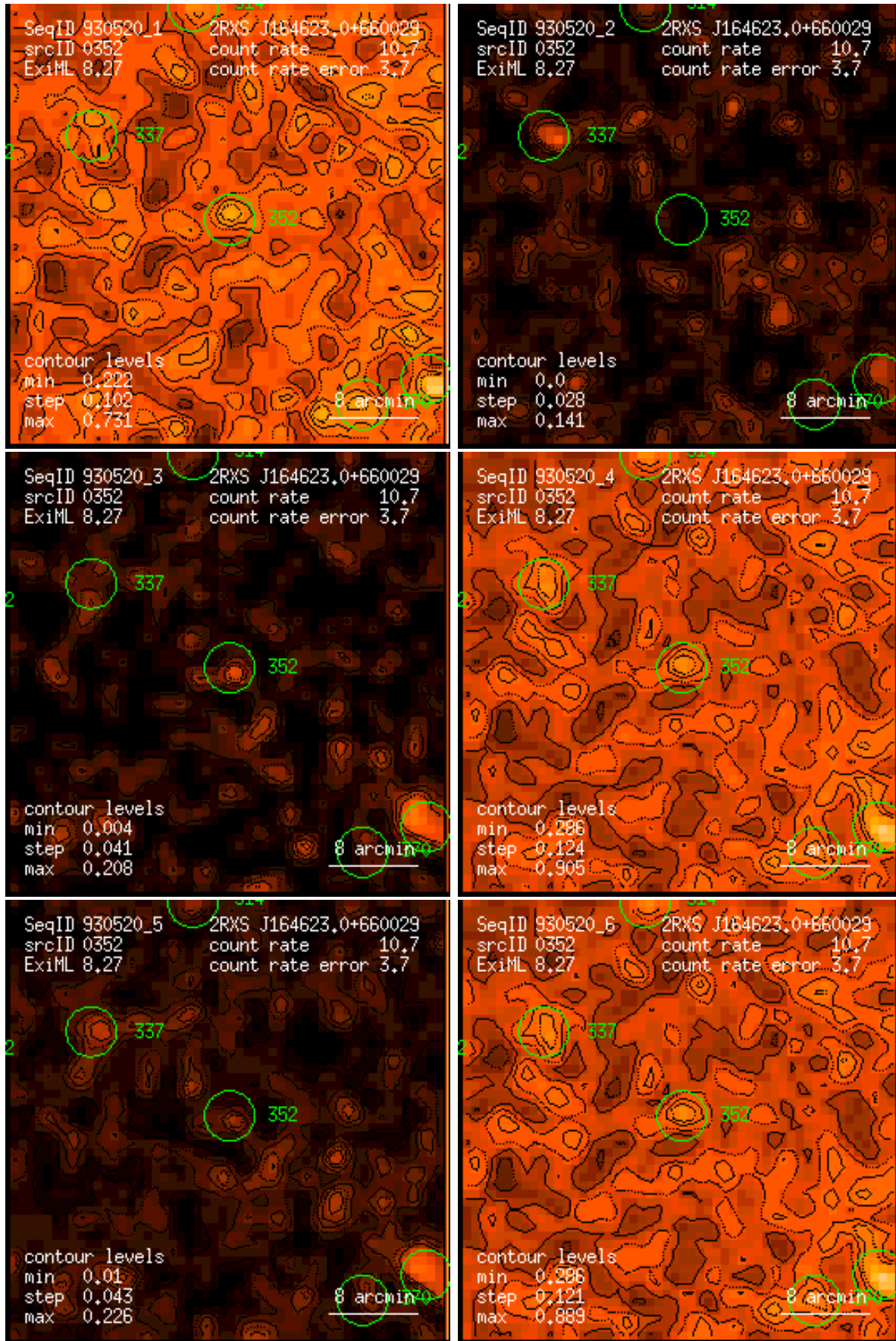
Figure 352: RASS 930520: detection 0352: band rate images, Gaussian filter: (1) PSPC channels 11 – 41, (2) 52 – 90, (3) 91 – 201, (4) 11 – 235, (5) 52 – 201, (6) 11 – 201. Broad band rates in counts/ks. Band rate contour levels in counts/ks/arcmin 2 .
